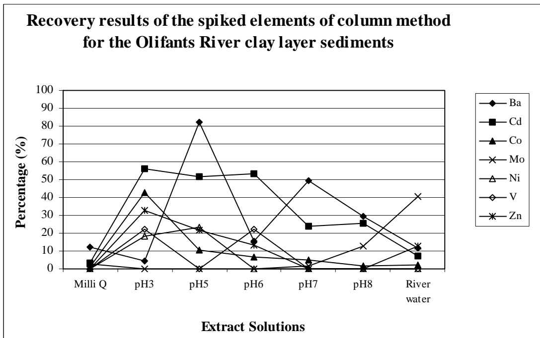
Graph 3. Recovery results of the spiked elements of column method for the Olifants River clay layer sediments.
