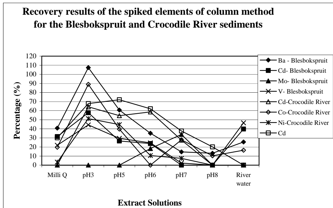
Graph 1. Recovery results of the spiked elements of column method for the Blesbokspuit and Crocodile River sediments
