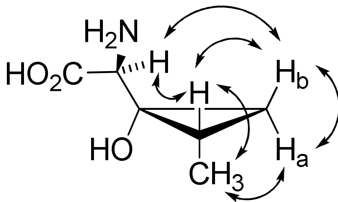
Figure 2. NOE connectivity pattern observed for diplonine (1).
