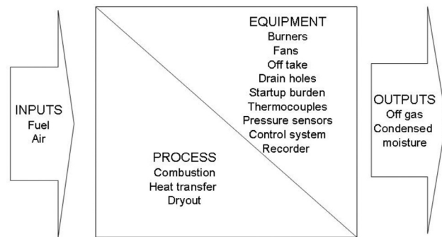
Figure 2—Analysis of the dryout process
