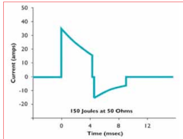
Figure 6: A typical BTE waveform
