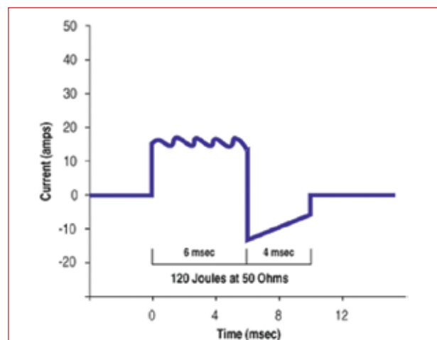
Figure 7: A typical rectilinear biphasic waveform
