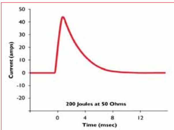
Figure 5: A typical monophasic waveform
