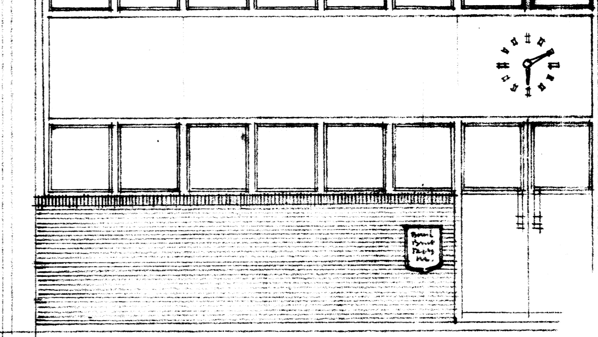
STREET ELEVATION. (Showing Brick DADO and new)
