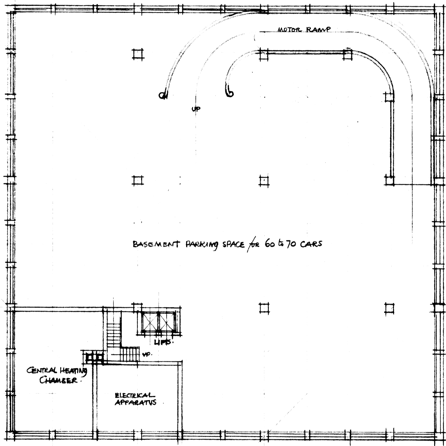
BASEMENT PLAN .
