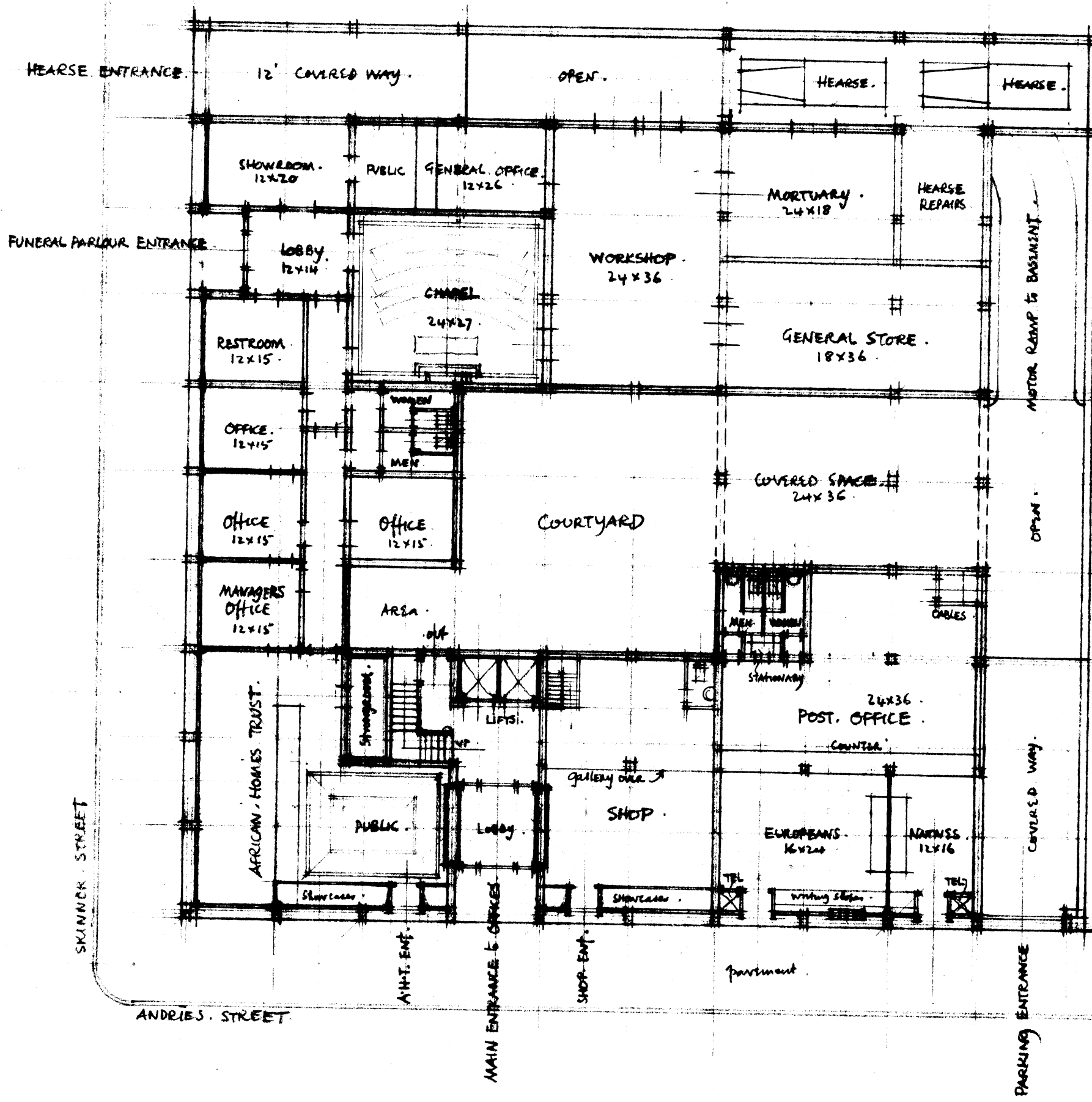
PROPOSED NEW BUILDING for AFRICAN HOMES TRUST and INSURANCE CO. LTD. PRETORIA. SIXTEENTH SCALE SKETCH PLAN. DRAWING NO P.176/1.A 26:10:44. Norman Eason & Partners. ARCHITECTS. PRETORIA.
