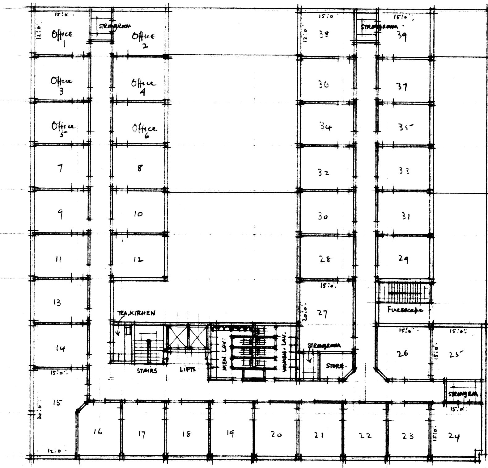
FIRST and UPPER FLOOR PLANS .
