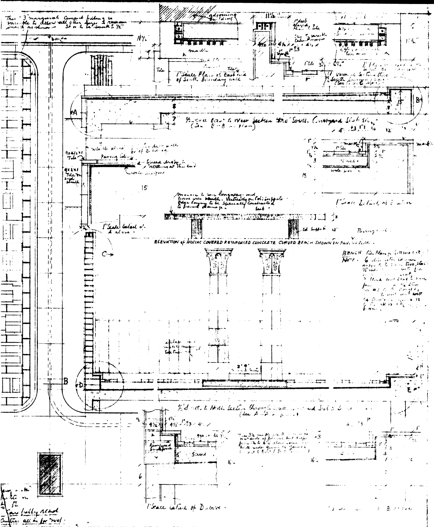
PAVED SOUTH GROUND FLOOR SHOWING MOSAIC AND OLD ARCADE MEMORIAL MOSAIC & COLUMNS. SCALE 1/2" = 1 FOOT. DATE MAR. 1965
