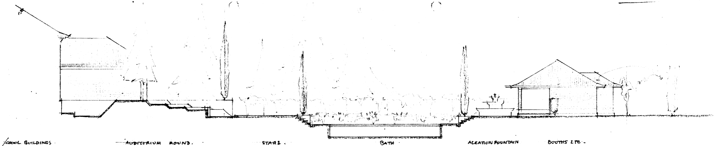
NORTH TO SOUTH LONGITUDINAL SECTION.
