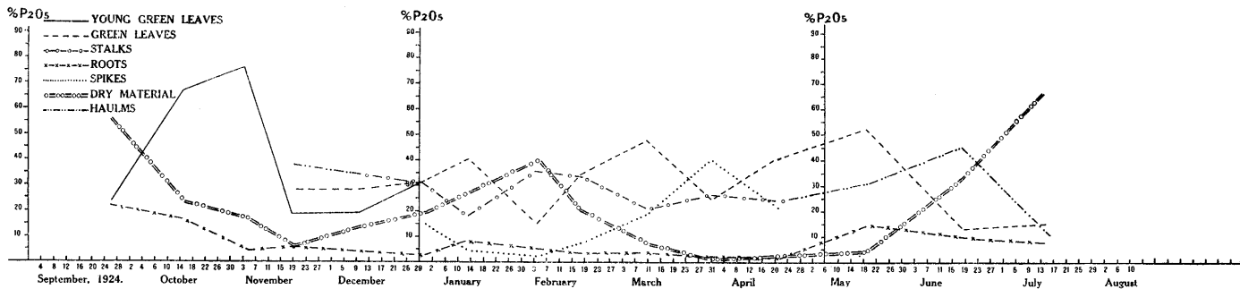
CHART 25.— Eragrostis lehmanniana .
