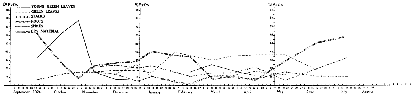
CHART 16.— Eragrostis superba .
