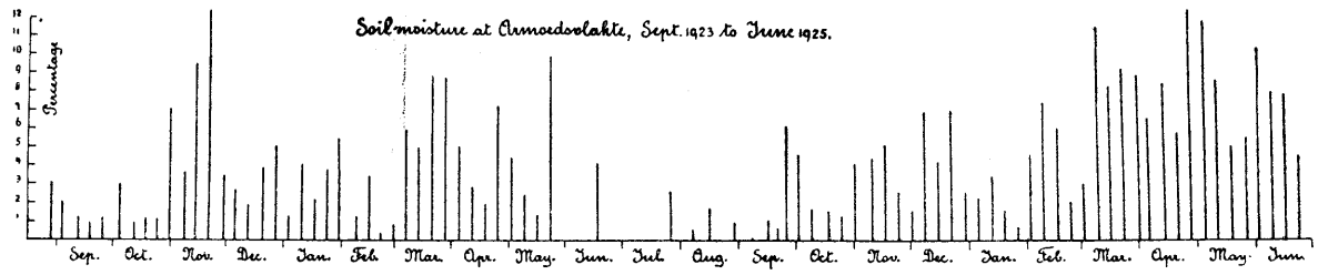
CHART 51.
