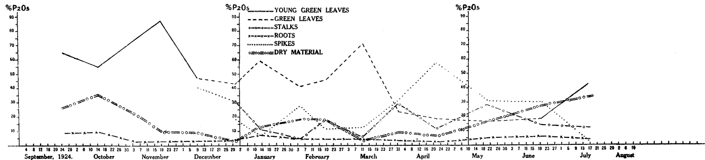
CHART 22.— Aristida congesta .
