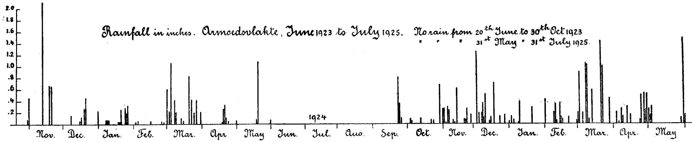
CHART 50.
