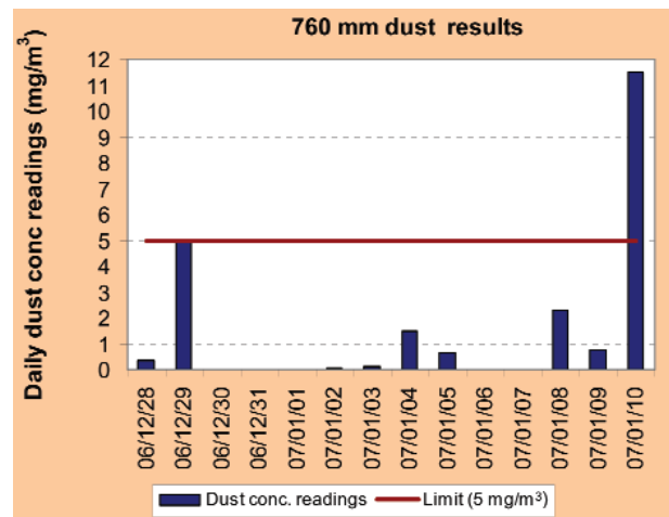
Figure 18—Rear-exit scrubber results
