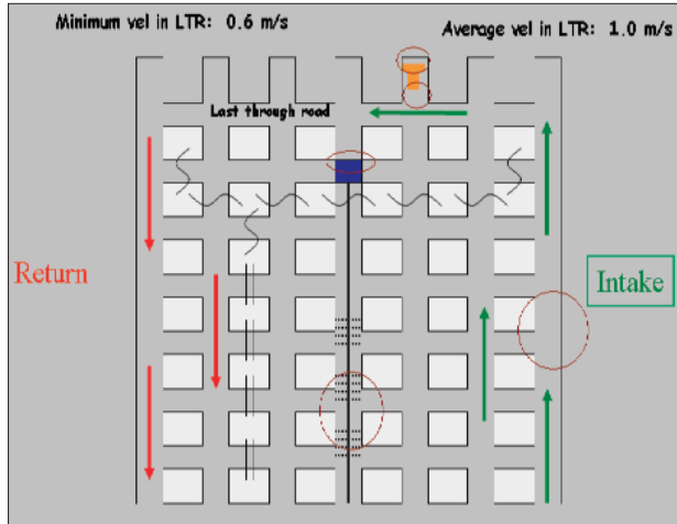
Figur 24—A typical 7 road section showing dust sources circled in red and basic ventilation
