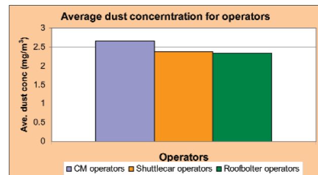
Figure 9—Personal sampling for Sasol mining operators
