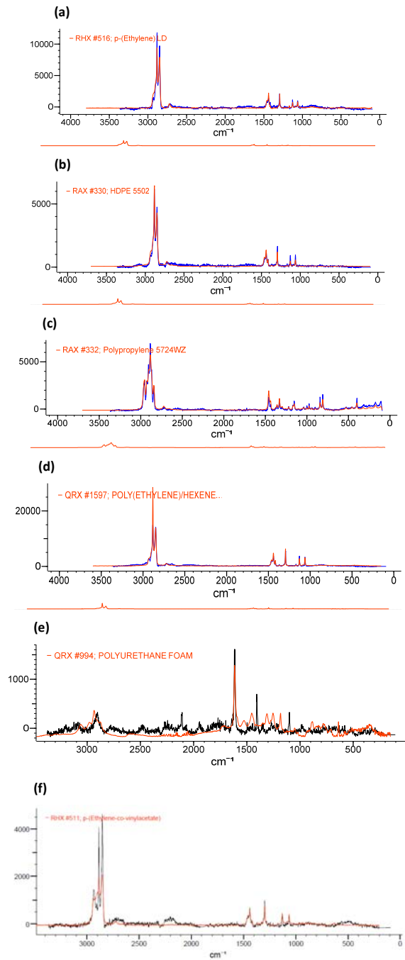
Fig. S1 Raman spectra of (a) LDPE, (b) HDPE, (c) PP, (d) Poly(ethylene-co-1-hexene) copolymer, (e) Polyurethane, and (f) Poly(ethylene co-vinyl acetate).
