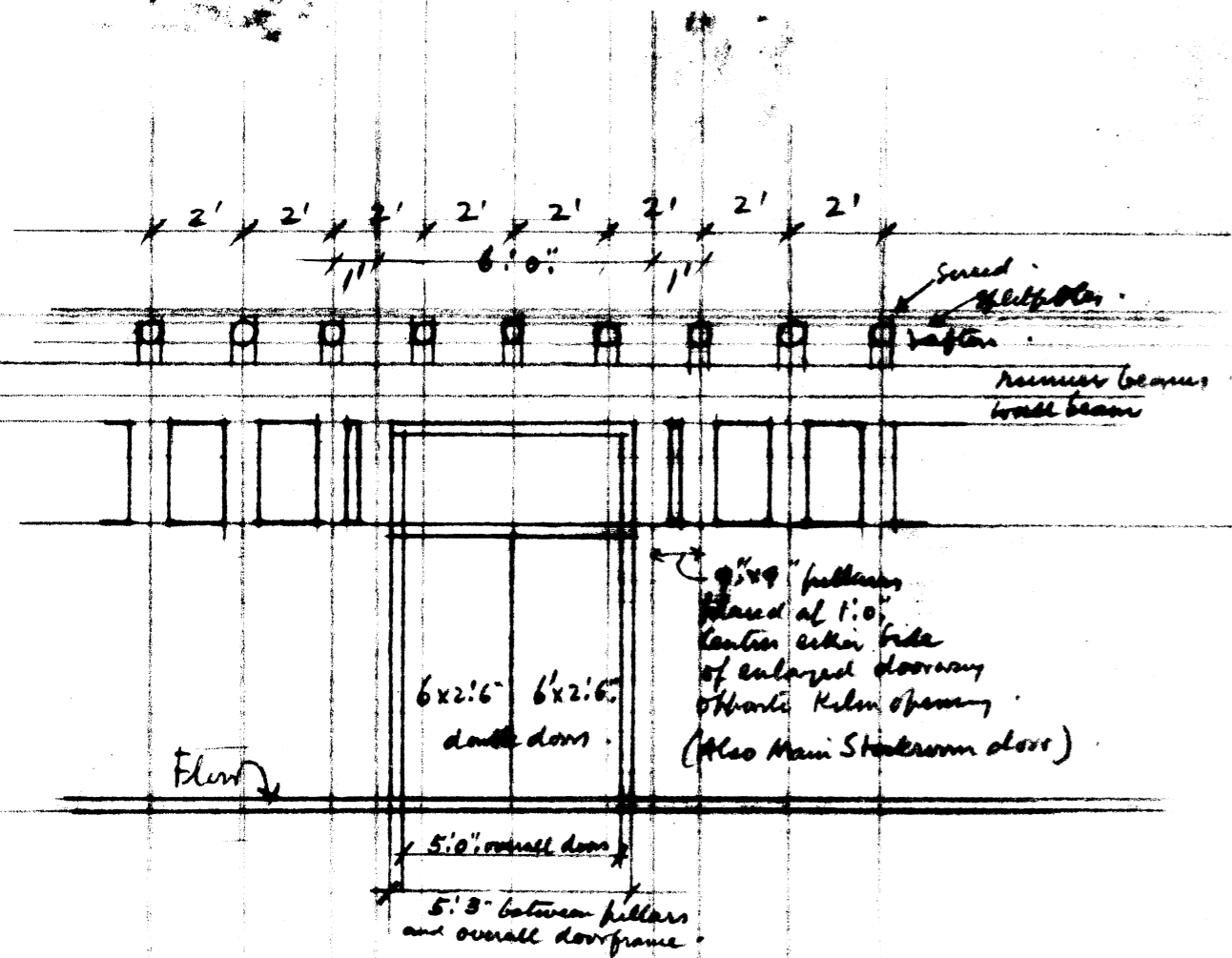
EAST TO WEST SECTION SHOWING METHOD OF ENLARGING SOUTH KILNHOUSE DOOR.
