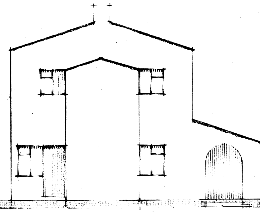
east elevation
