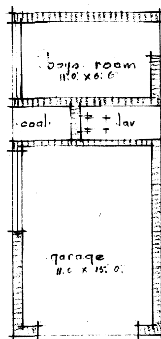
outbuildings plan
