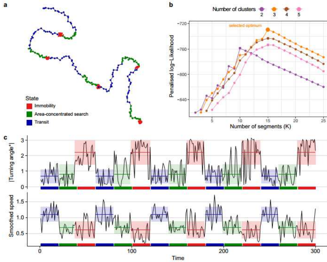
Fig. 3. Example of application of the segclust2d/segmentation-clustering procedure to highlight behavioural changes in a simulated movement. (a) Simulated path as a composite correlated random walk, incorporating an additional noise with standard deviation \zeta = 0.3 u that affects locations; (b) Determination using BIC-based penalised likelihood of the most likely numbers of states ( M = 3 ) and segments ( K = 15 ) (big orange dot), and of the most likely number of segments for the other three numbers of states considered (large squares at the top of the curves). (c) Corresponding time-series in terms of absolute turning angle computed with a constant step length, |\alpha_i^*| , and smoothed speed, (L_i + L_{i+1}) / (2\Delta t) , segmented with L_{min} = 10 and M = 3 ; the coloured bands appearing over the two time-series show the estimated occurrences and mean (plain horizontal line running in the middle of the band) \pm standard deviation (band width) for each of the three movement modes whereas the horizontal colour bars running along the time axis show the true occurrences of these modes.
