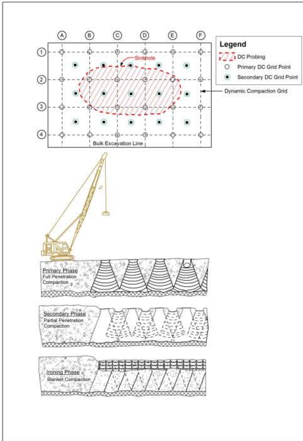
Figure 2. Schematic depiction of a Dynamic Compaction grid layout and compaction patterns for Dynamic Compaction Probing, primary, secondary and ironing phases (modified after Byrne et. al., 1995).
