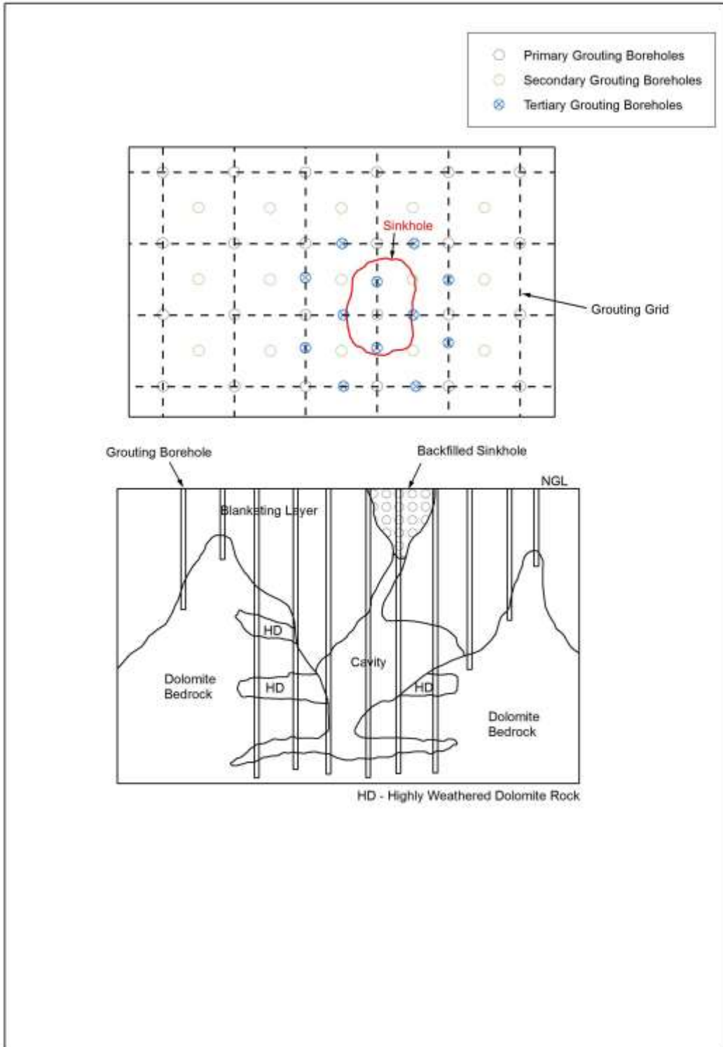
Figure 3. Schematic depiction of a grouting grid comprising primary, secondary and tertiary grouting points to rehabilitate a sinkhole.
