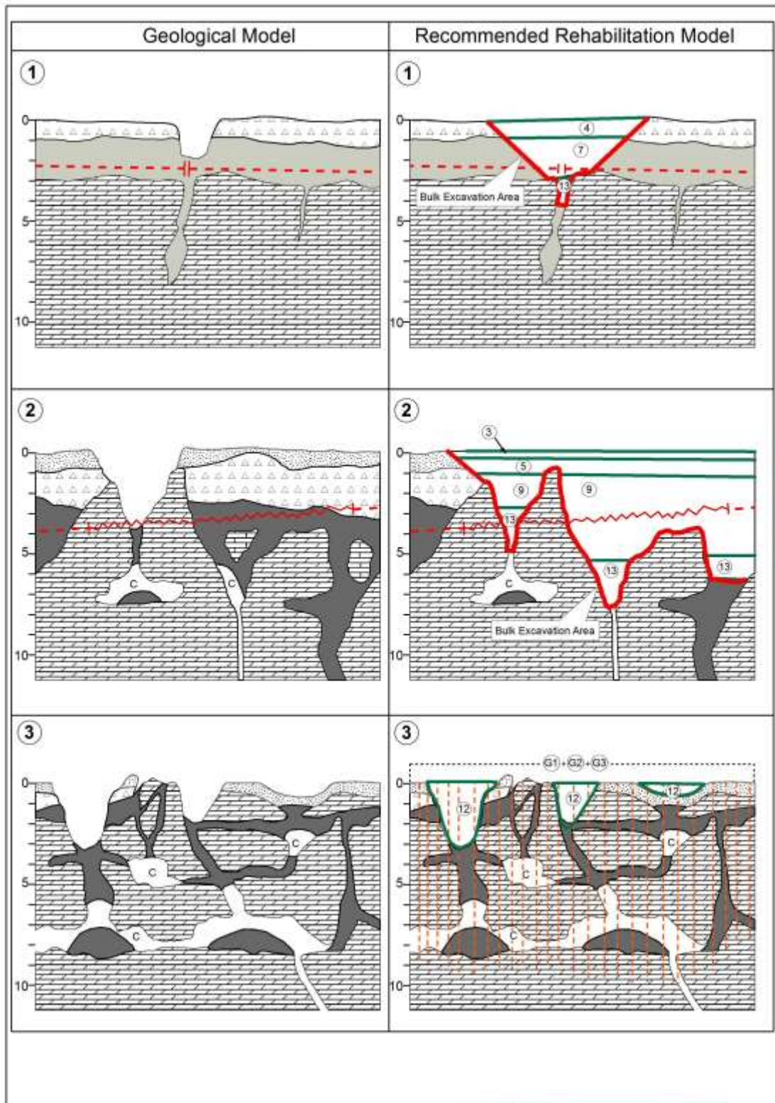
Figure 4. Generic Geological and Rehabilitation Model 1 to 3.
