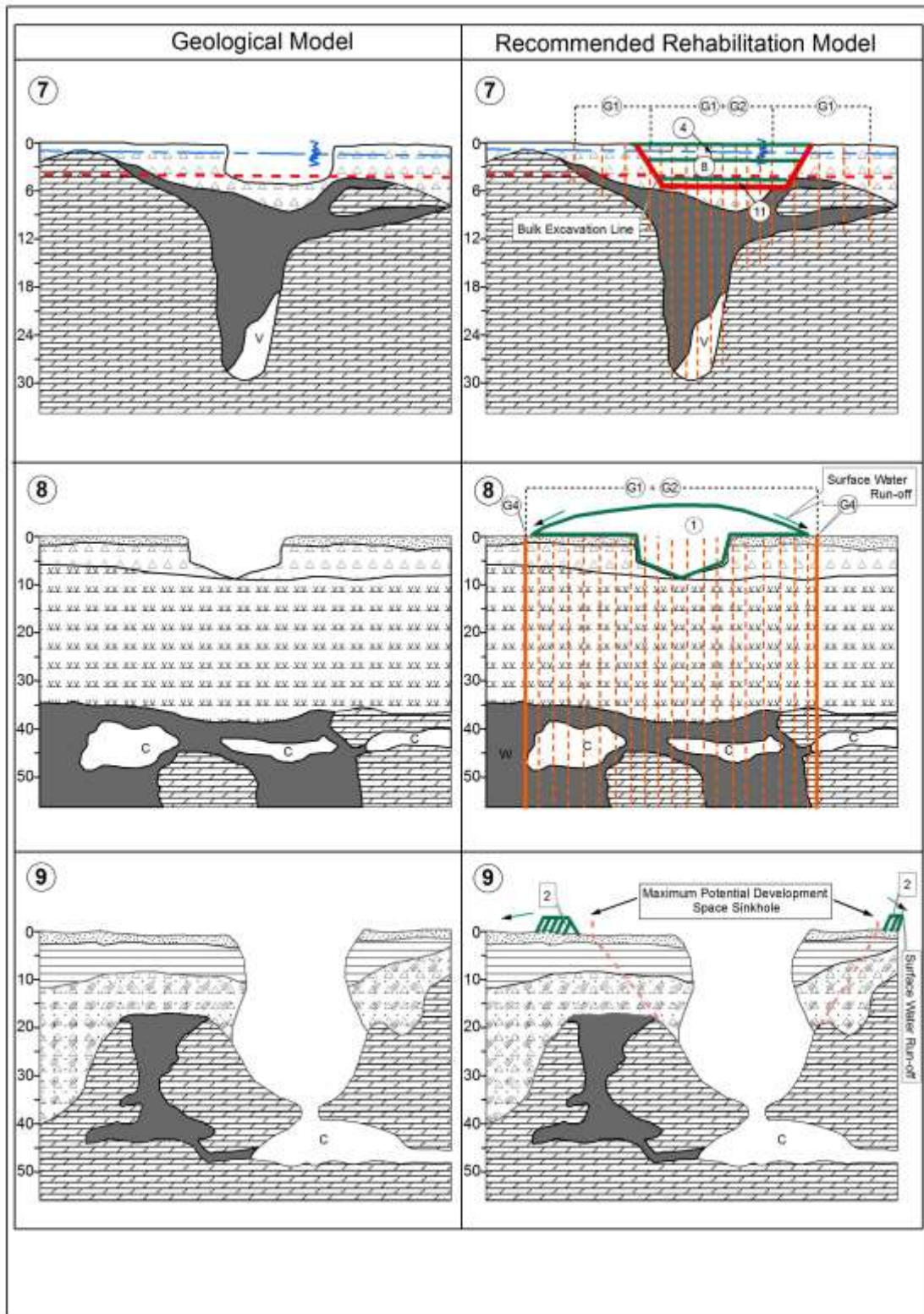
Figure 6. Generic Geological and Rehabilitation Model 7 to 9.
