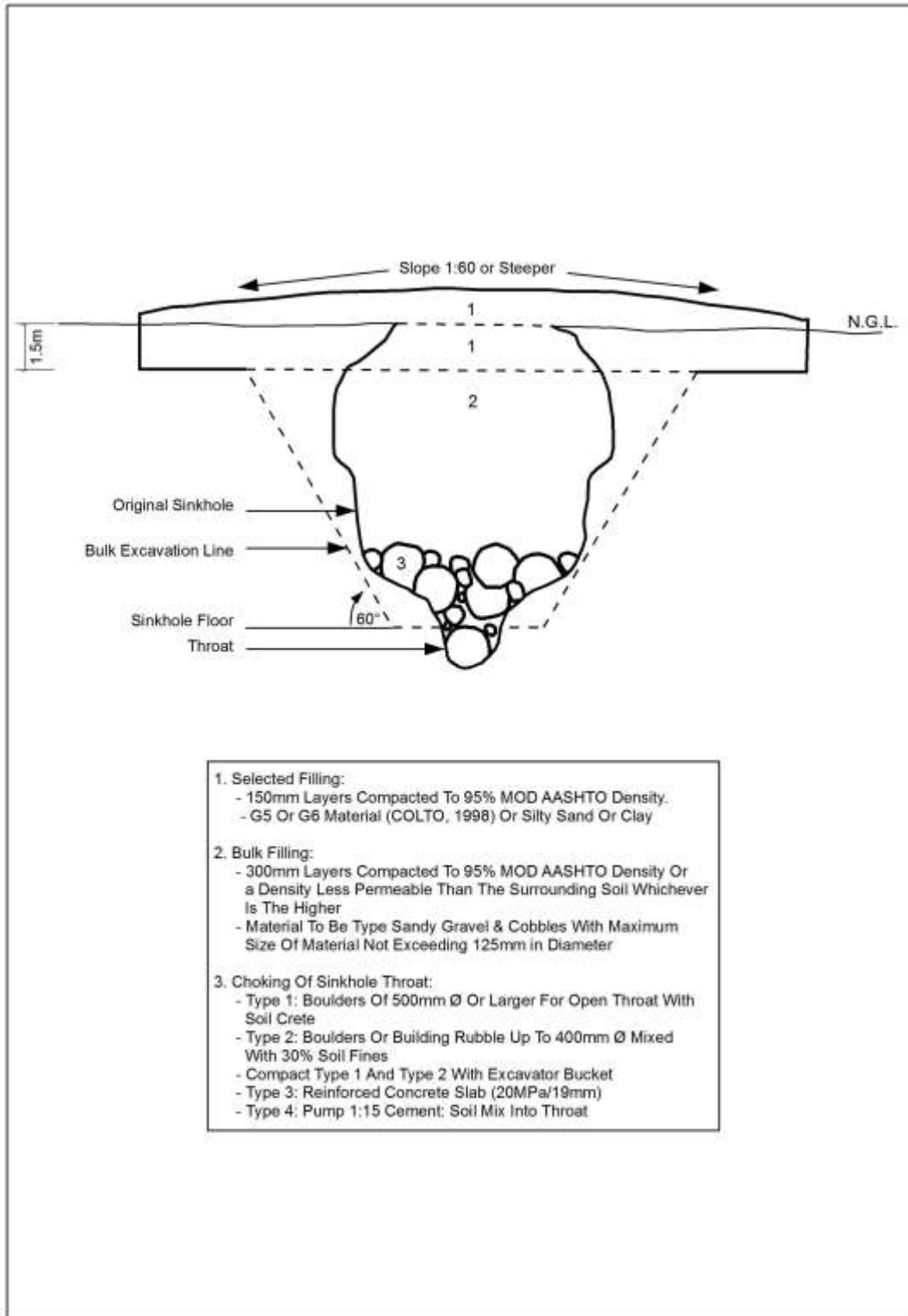
Figure 1. Schematic depiction of the Inverted Filter Method used to rehabilitate a sinkhole (modified after PW344, 2010).
