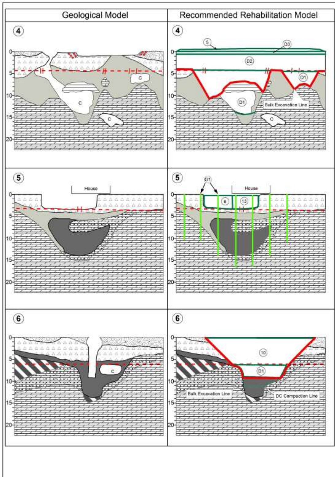
Figure 5. Generic Geological and Rehabilitation Model 4 to 6.
