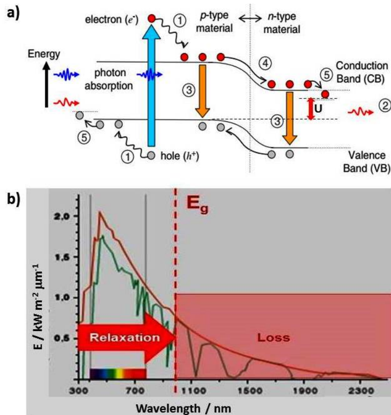
Figure 14: a) Loss processes in a semiconductor photovoltaic cell: 1) lattice thermalisation loss (internal conversion), 2) non-absorption of below band gap photons, 3) recombination losses, 4) and 5): junction and contact voltage loss, U : usable voltage. b) The Shockley-Queisser limit for a given band gap energy E_g originates in loss processes due to non-absorption of below band gap photons (red hashed range, 2) in part a), and to relaxation processes 1), 4), and 5). (a) Reprinted from Ref. 17, copyright (2006), with permission from Elsevier. (b) Reprinted with permission from Ref. 18.
