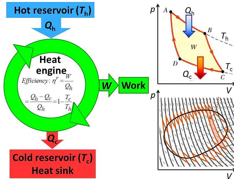
Figure 8: The heat engine operates between a high temperature reservoir, the combusting fuel, and a low temperature reservoir, the cooling system which acts as a heat sink for the waste heat that is inevitable when the machine produces work. The process of the machine is explained by the Carnot cycle (upper right), consisting of a sequence of isothermic and adiabatic steps. In a p - V diagram, the area of the cycle represents directly the work W provided by the process. Any cyclic process can be thought of consisting of multiple infinitesimal Carnot cycles, the conclusions reached for the simple cycle are therefore general.
