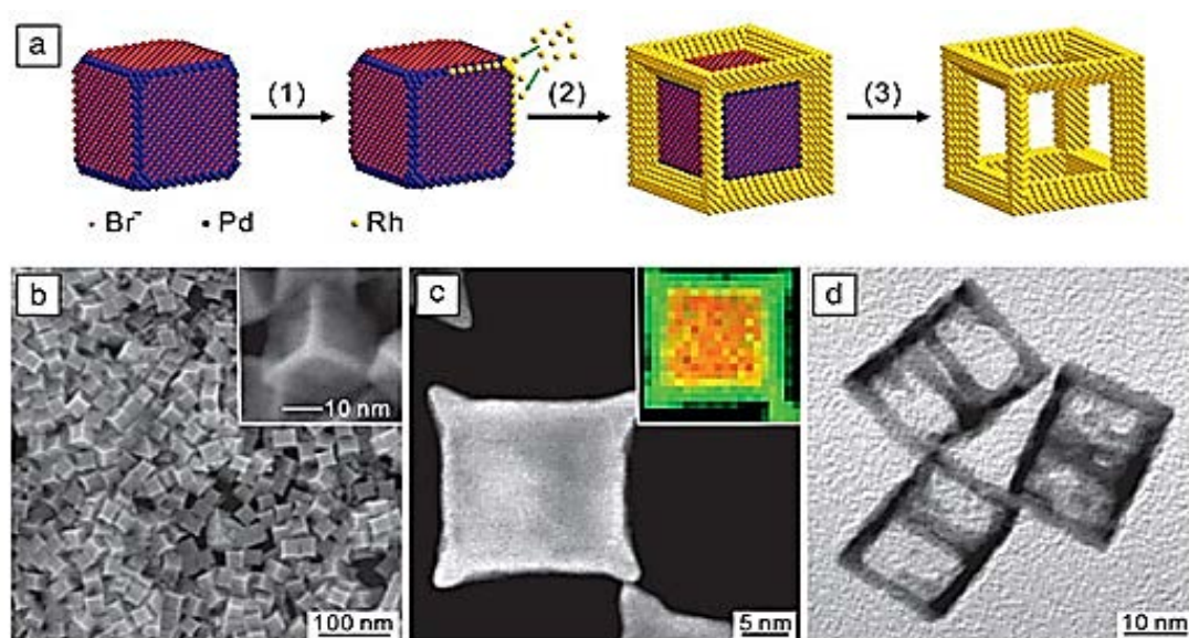
Figure 19: a) Synthesis of cubic rhodium nanoframes by site-selective overgrowth of Pd nanocubes and selective etching of the Pd nanocores. 29 b) scanning electron microscopy image of Pd-Rh core-frame nanocubes, c) transmission electron microscopy and element-selective, energy-dispersive X-ray mapping (inset) of an individual core-frame nanocube, d) transmission electron microscopy image of Pd-etched rhodium nanoframes (Y. Xia, X. Xia, Y. Wang, S. Xie, Shape-controlled synthesis of metal nanocrystals, MRS Bulletin, 38, 2013, 335-344, reproduced with permission.).
