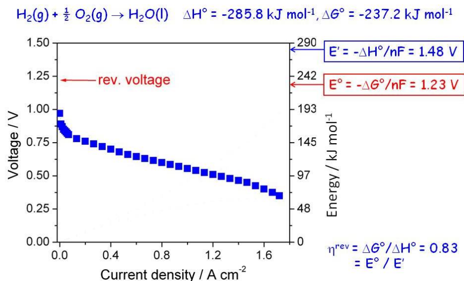
Figure 6: Polarisation curve of a polymer electrolyte hydrogen fuel cell as a function of the current density.
