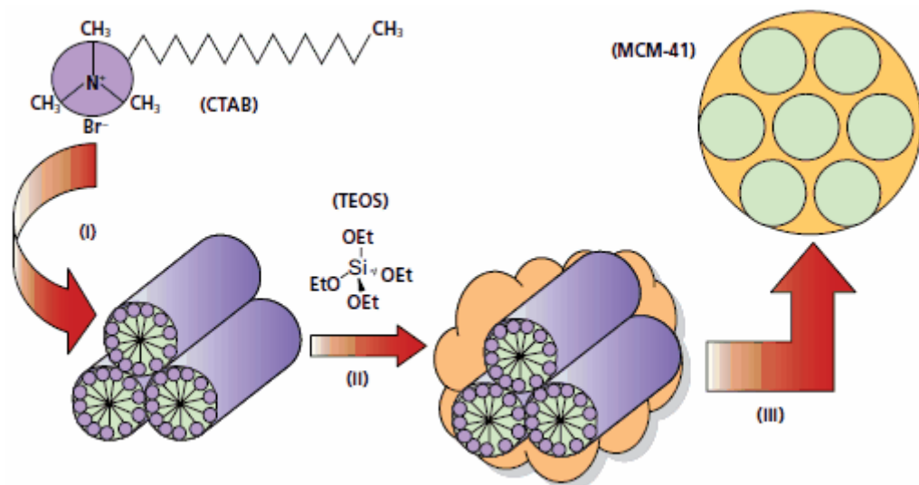
Figure 20: Surfactants, here cetyltrimethylammonium bromide (CTAB) form a rich variety of soft matter structures which are used as templates for the sol-gel process of alkoxides, here tetraethylorthosilicate (TEOS), which is hydrolysed, followed by condensation to the template-directed silica structure and subsequent burning off of the organic phase (Reproduced from Ref. 30).
