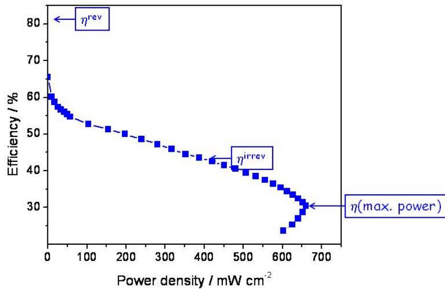
Figure 7: Efficiency of the hydrogen fuel cell (data from Figure 6) as a function of the electrical power density (the product of actual voltage and current density).
