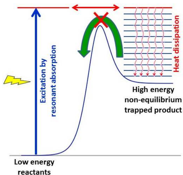
Figure 13: Basic scheme showing the key mechanism of stabilising a high-energy product state that is trapped behind a barrier following excitation by resonant absorption of light. Heat dissipation in a bath makes sure that the energy barrier back to the reactants can no longer be crossed at thermal energies. The barrier intercepts the arrow of time. Pumped hydro-storage might be regarded as a macroscopic analogue of the mechanism.
