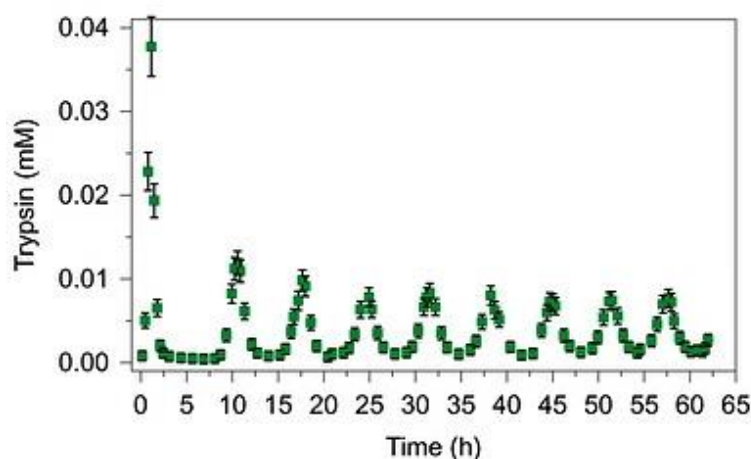
Figure 3: Pronounced sustained oscillation of the concentration of the enzyme trypsin with a period of 6.5 h in an artificially constructed tuneable dissipative chemical reaction network (Reprinted with permission from Macmillan Publishers Ltd: Nature Chemistry (Ref. 6), copyright (2015)).
