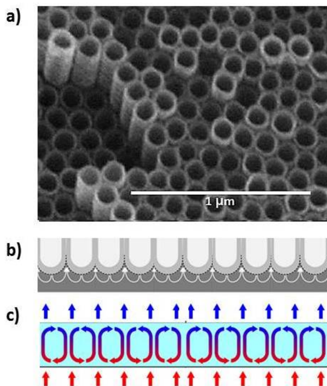
Figure 21: a) Hexagonal array of TiO 2 nanotubes grown by anodisation of a Ti foil. 32 b) Suggested plastic flow that leads to dissolution of Ti foil and formation of nanotubes. 33 c) Rayleigh-Bénard convection cells develop in a gravitation field when a thin layer of a liquid is heated smoothly from below and cooled from above. The alternating clockwise and counter-clockwise rotation of the developing cells is a consequence of instabilities leading to spontaneous symmetry breaking and self-organisation to new order in the heat gradient. (a) Reprinted from Ref. 32, copyright (2010) John Wiley & Sons, Inc. (b) Reprinted from Ref. 33, copyright (2011), with permission from Elsevier.
