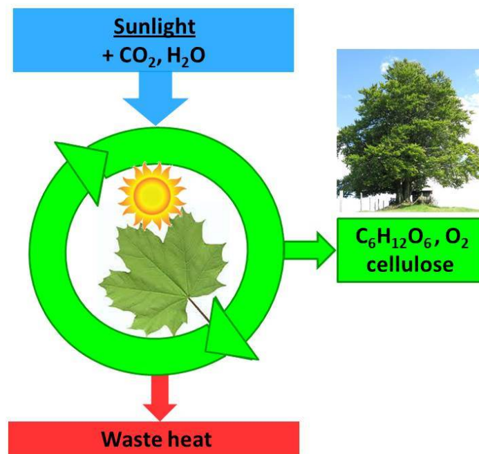
Figure 17: Photosynthesis can generate non-equilibrium low entropy glucose and cellulose only because it dissipates waste heat.
