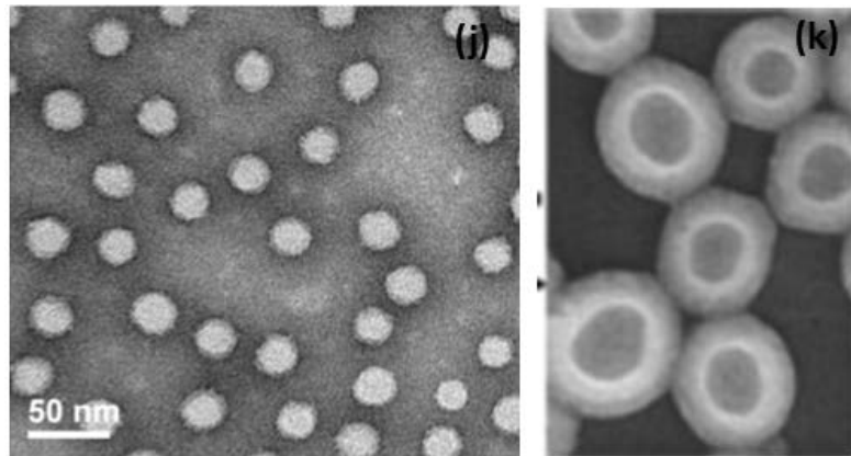
Figure 23: A representation of (a) an amphiphile, (b) a surfactant, (c) a lipid molecule, (d) an amphiphilic diblock copolymer; the structures formed by an amphiphile (e) Langmuir monolayer at the air-water interface, (f) a micelle, (g) an inverted micelle, (h) a bilayer, (i) a vesicle; transmission electron micrographs of (j) micelles formed from \text{PSMA}_{100}\text{-}b\text{-PS}_{250} , (k) \text{PS}_{300}\text{-}b\text{-PAA}_{44} , amphiphilic diblock copolymers
