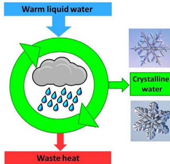
Figure 11: Crystallisation from gas phase or from solution leads to a lower entropy, ordered crystalline state and requires the dissipation of the heat of crystallisation. The two snowflakes have the same crystal structure of hexagonal ice despite their different morphologies.
