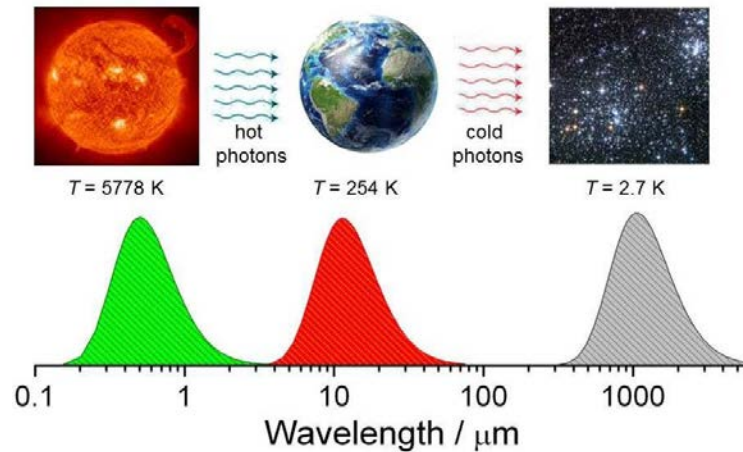
Figure 12: The fundamental gradient which drives life on earth. The formation of organic matter from carbon dioxide and water and its reproduction is made possible by a complex process called photosynthesis.
