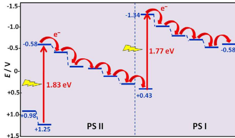
Figure16: Electron transfer cascades in the photosynthetic reaction centres PS I and PS II (adapted from Ref. 20).
