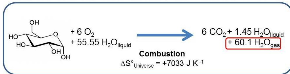
Figure 18: Although in our daily experience glucose is stable for years it is in reality thermodynamically unstable and undergoes spontaneous combustion to CO 2 and H 2 O in the presence of molecular oxygen. In a closed system (a) the heat of reaction is dissipated to the environment. If we regard this system as a model universe, place it in liquid water and isolate it (b) then the heat of reaction heats up the water and evaporates most of it. The entropy increase of the model universe is much larger than the entropy of reaction of the system.
