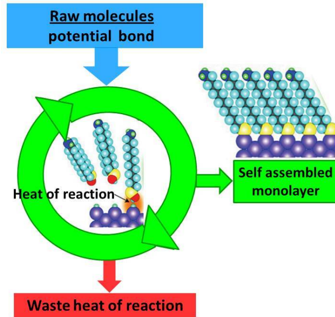
Figure 22: The heat of reaction that is liberated during spontaneous self-assembly of supramolecular structures has to be dissipated.
