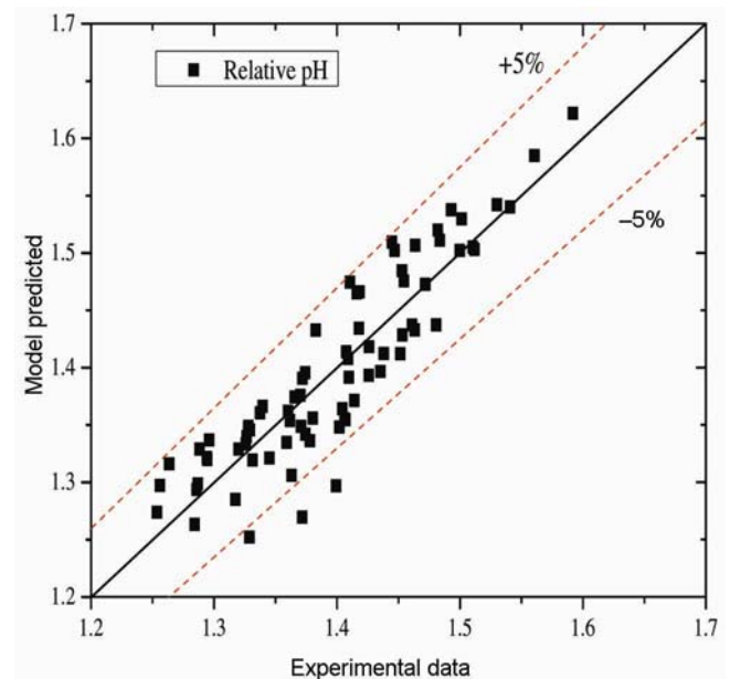
Figure 13. Parity plot between the predicted and experimentally measured pH data.
