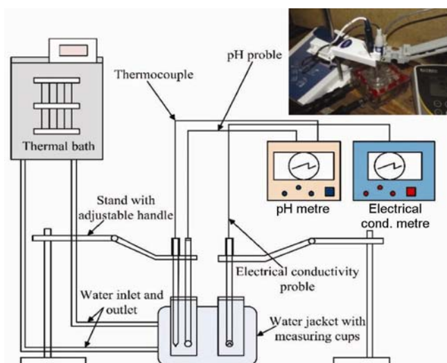
Figure 1. Schematic of the experimental set-up with inset showing the pictographic of the measurement site.
