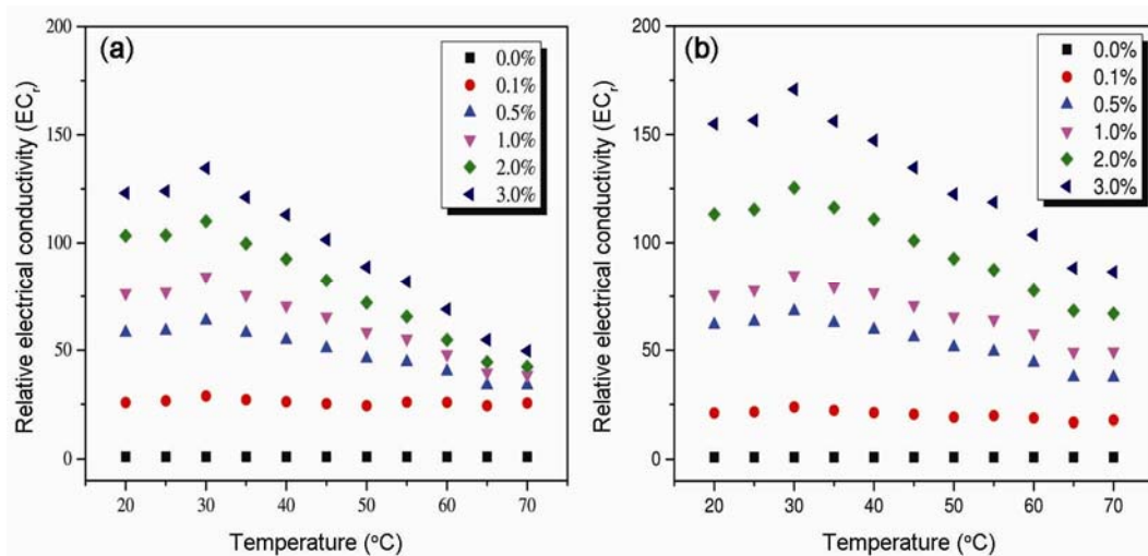
Figure 8. Relative electrical conductivity of MgO–EG nanofluid against temperature: (a) MgO-20 and (b) MgO-100.
