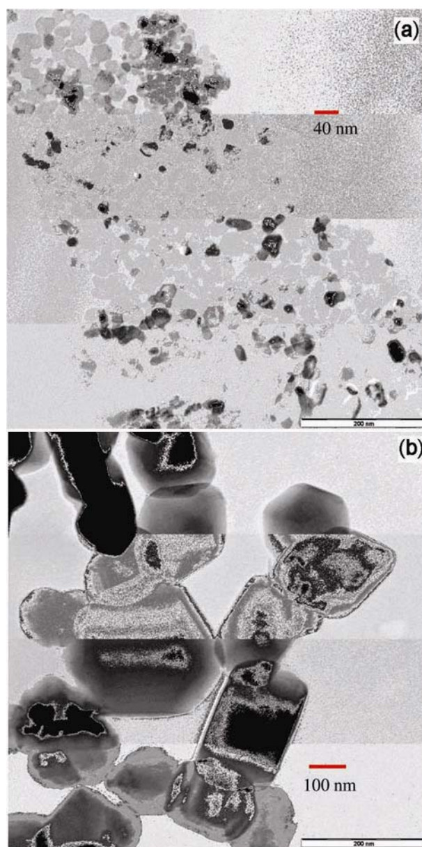
Figure 2. TEM image of MgO nanoparticles: (a) MgO-20 and (b) MgO-100.
