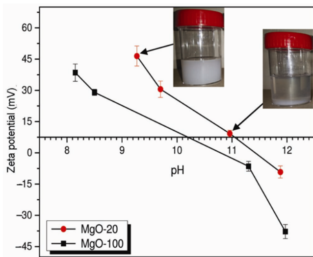
Figure 5. Zeta potential ( \zeta ) of MgO–EG nanofluids as a function of pH modified by KOH and/or HCl.
