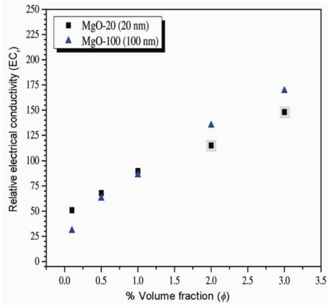
Figure 10. Effect of the volume fraction on the relative electrical conductivity of MgO-EG at room temperature.
