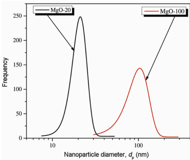
Figure 3. MgO nanoparticles size distribution.
