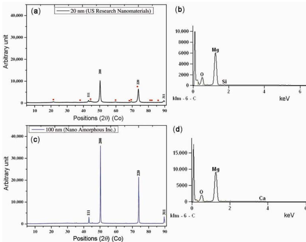
Figure 4. XRD and EDS spectral patterns of MgO nanoparticles: (a and c) XRD spectral of MgO-20 and MgO-100 nm, respectively and (b and d) EDS spectral of MgO-20 and MgO-100 nm, respectively.
