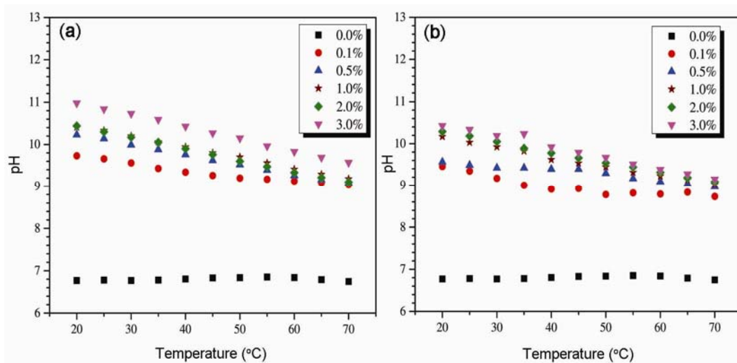
Figure 6. Influence of temperature on the pH of MgO-EG nanofluid: (a) MgO-20 and (b) MgO-100.
