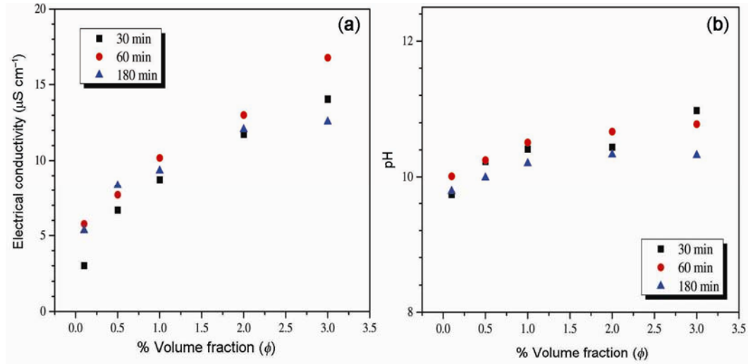
Figure 12. Influence of ultrasonication time/energy density on the electrical conductivity and pH of MgO-EG nanofluid at 20°C: (a) electrical conductivity and (b) pH.
