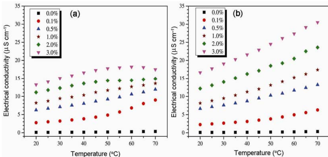
Figure 7. Influence of temperature on the electrical conductivity of MgO-EG nanofluid: (a) MgO-20 and (b) MgO-100.
