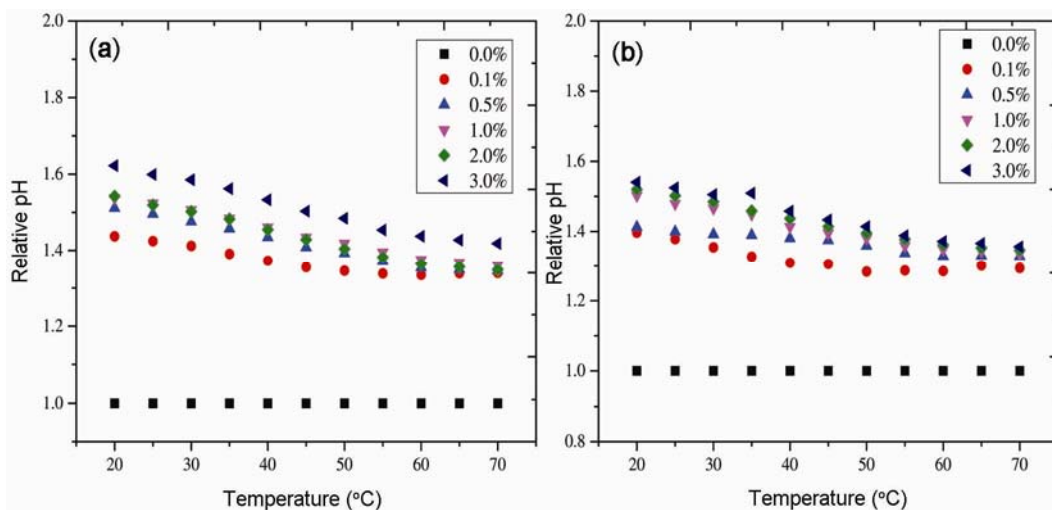
Figure 9. Relative pH of MgO–EG nanofluid against temperature: (a) MgO-20 and (b) MgO-100.
