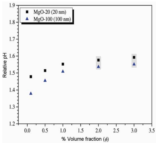
Figure 11. Effect of the volume fraction on the relative pH of MgO-EG at room temperature.
