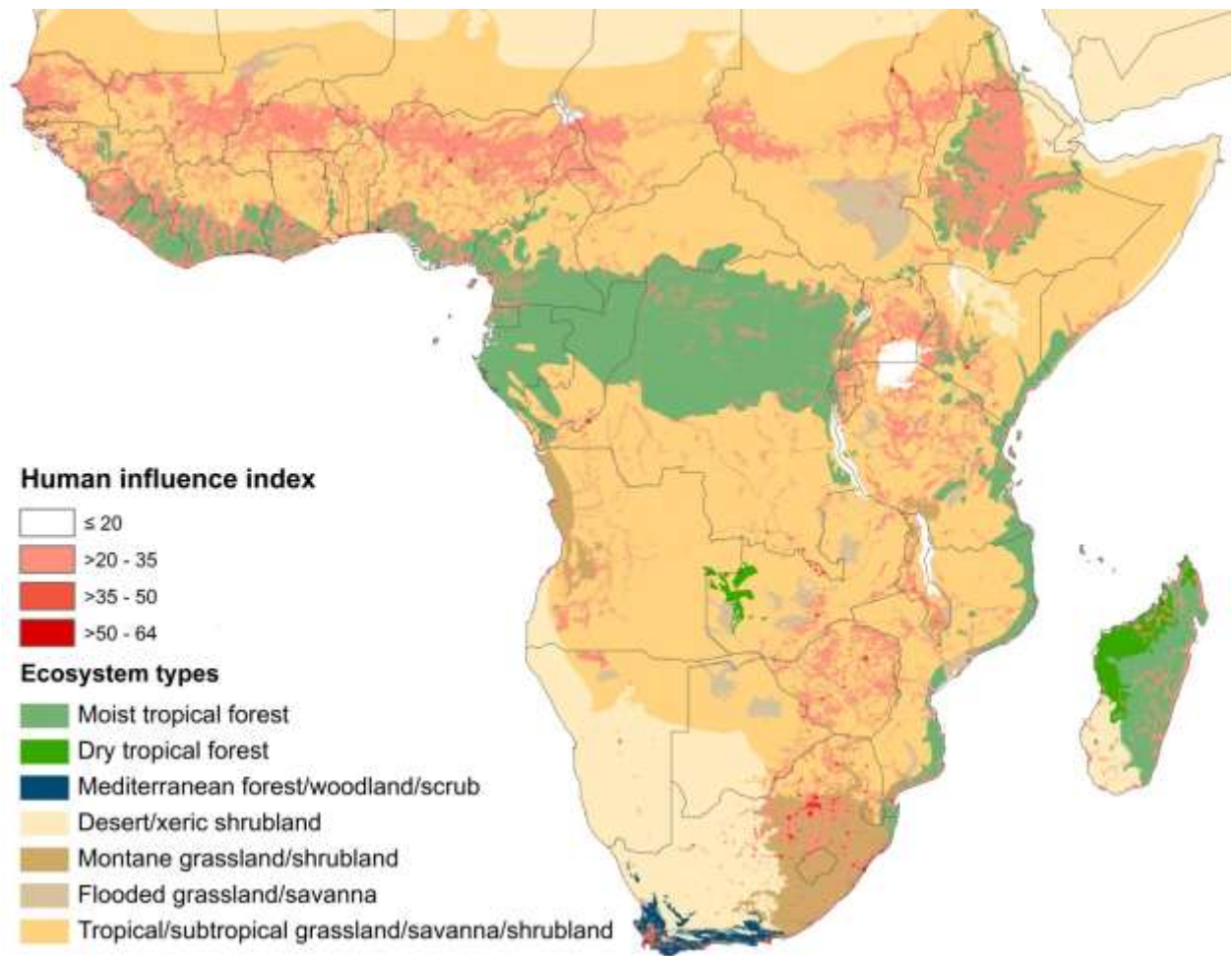
Figure 1. Map of sub-Saharan Africa showing ecosystem types adapted from Olson et al. (2001): rangelands (desert and xeric shrubland, montane grassland/shrubland, flooded grassland/savanna, and tropical/subtropical grassland/savanna/shrubland), tropical forests (moist and dry tropical forest), the Cape Floristic Region (Mediterranean forest/woodland/scrub), and the urban and rural built environment represented by the human influence index (Wildlife Conservation Society and Center for International Earth Science Information Network 2005), a dataset comprising nine data layers incorporating population pressure (population density), human land use and infrastructure (built-up areas, nighttime lights, land use, land cover), and human access (coastlines, roads, railroads, navigable rivers).
