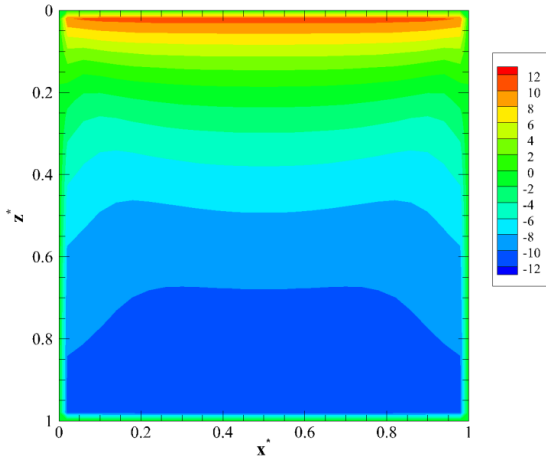
Figure 26: Contours of percentage difference in \nabla \cdot q_r(x^*, y^* = 0.5, z^*) between DOM with ballistic scattered energy normalization and Hunter and Guo's 2012 ballistic normalization for M = 80 in a tissue-mimicking medium
