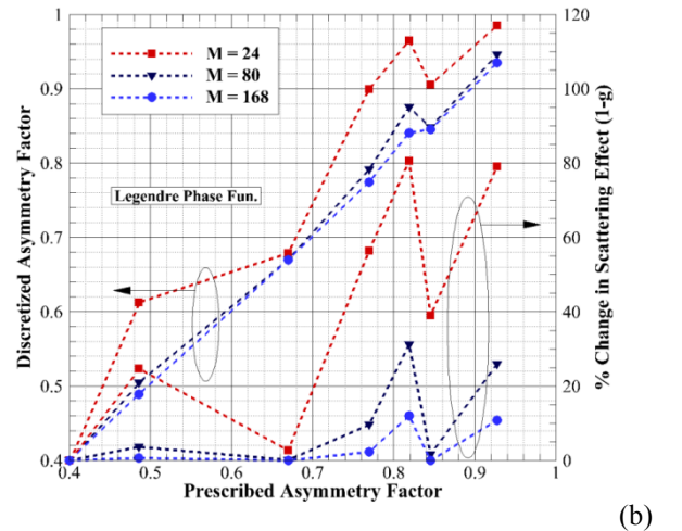
Figure 3: Comparison of discretized and prescribed asymmetry factor and change in scattering effect after application of scattered energy normalization for a) HG phase-functions and b) Legendre phase-functions
