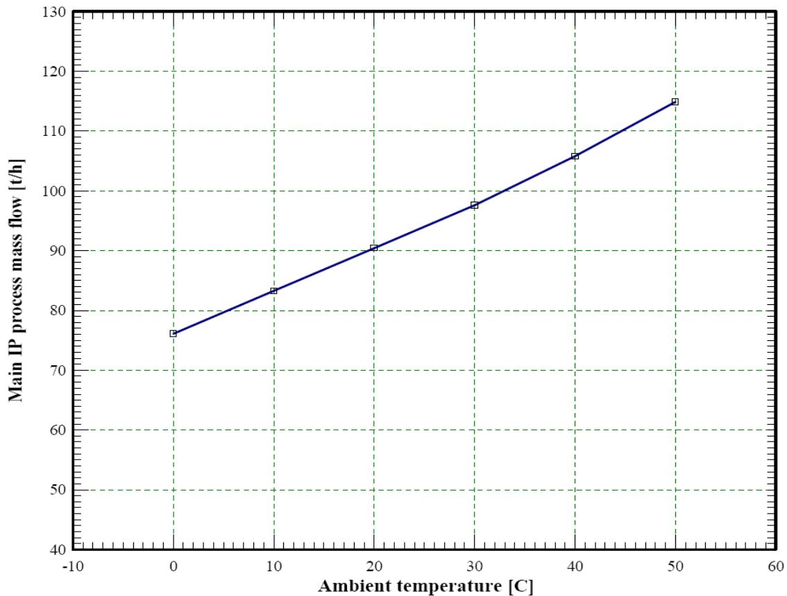
Figure 1. Influence of environment temp. on generated steam of HRSG
