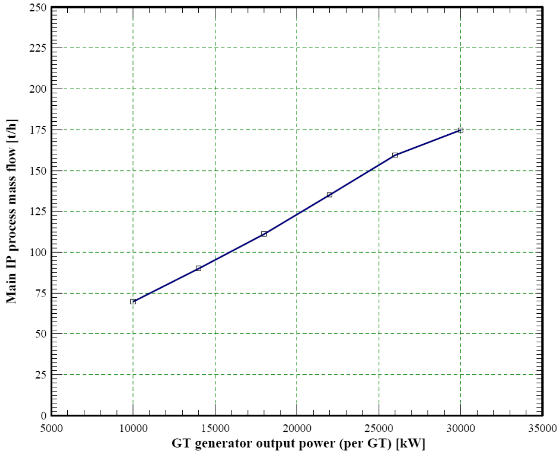
Figure 2. Influence of GTG power on generated steam of HRSG
