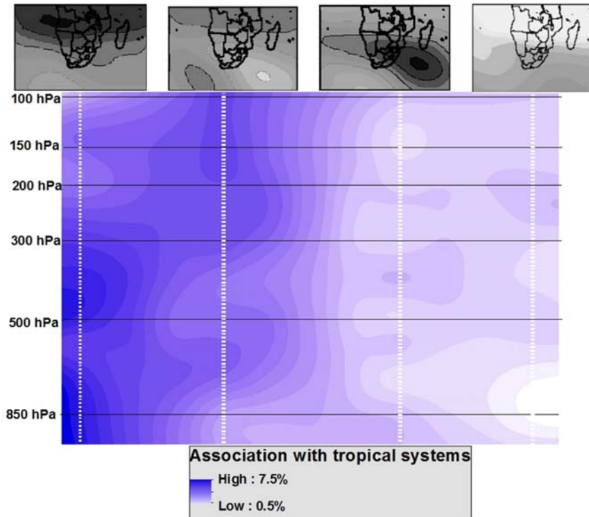
Fig. 3 Variation in concentration within each of the four SOM groups (indicated at the top) of landfall-event days per pressure level. The pressure levels are represented on the vertical from bottom (1000 hPa) to top (100 hPa).
