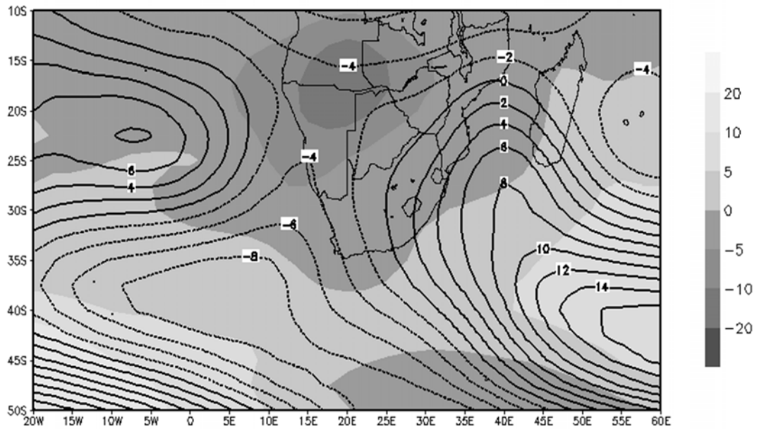
Fig. 5 850 hPa (shaded) and 250 hPa (contours) height anomalies (units: m) for the 1995-2002 period.
