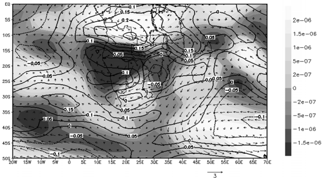
Fig. 10 Difference in 850 hPa relative vorticity (shaded, units: s^{-1} ), wind shear between 850 hPa and 200 hPa (black contours, units: ms^{-1}/km ) and wind vectors (scale shown) for the period 1995-2002 relative to the remaining years in the period 1979-2011.
