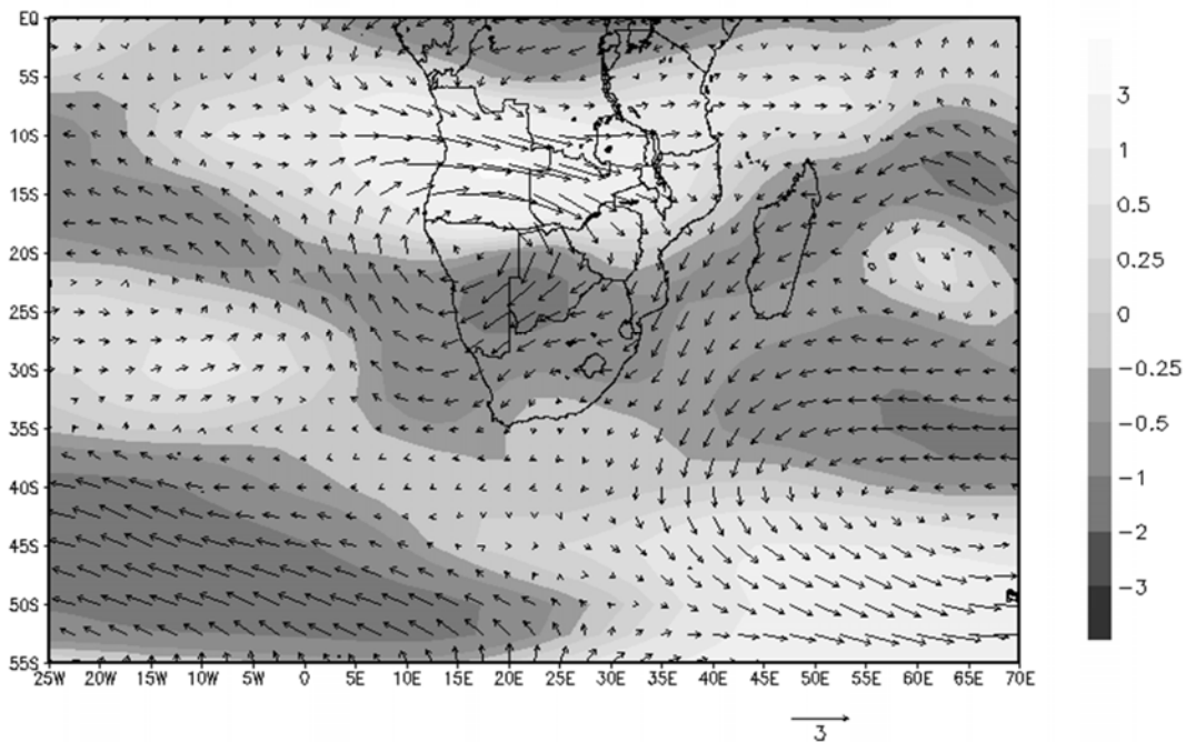
Fig. 8 Difference wind vectors (scale shown, units: \text{ms}^{-1} ) of the 700-500 hPa flow for the period 1995-2002 (difference in zonal component shaded, units: \text{ms}^{-1} ) compared to the rest of the 1979-2011 period.
