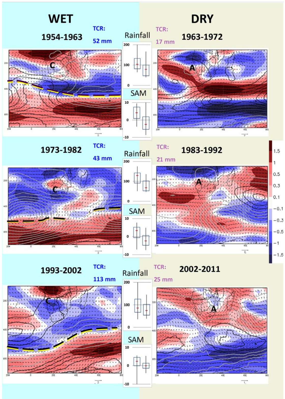
Fig. 14 500-700 hPa steering flow anomaly vectors (scale in \text{ms}^{-1} shown for each map) with U-component shaded (red – positive, blue – negative, units: \text{ms}^{-1} ), and 250 hPa height anomalies (contours) for alternating wet (left) and dry (right) multi-year epochs as indicated. Contour intervals are 5 m; dark (light) contours are for negative (positive) anomalies. The positions of prominent ridges at 850 hPa are also indicated (broken black/yellow lines). Inter-quartile ranges for rainfall (units: % of average during JFM) as average for all 8 stations in Fig. 1 and the SAM are indicated per epoch for comparison in box plots. The average annual rainfall contributed by tropical systems (TCR, units: mm) from the SWIO calculated as an average for the eastern stations (dark circles in Fig. 1) is also indicated per epoch.
