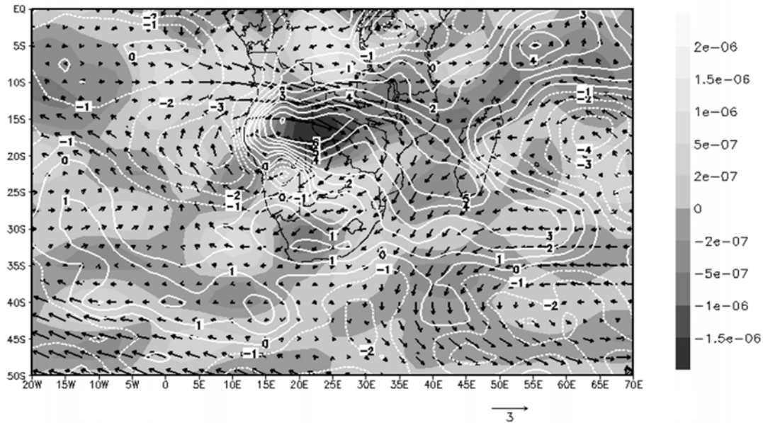
Fig. 9 Difference in 850 hPa convergence (shaded, units: s^{-1} ) and difference in relative humidity at 600 hPa (white contours, units: %). 850 hPa wind vector anomalies for the period 1995-2002 relative to the remaining years in the period 1979-2011 are also indicated (scale shown).
