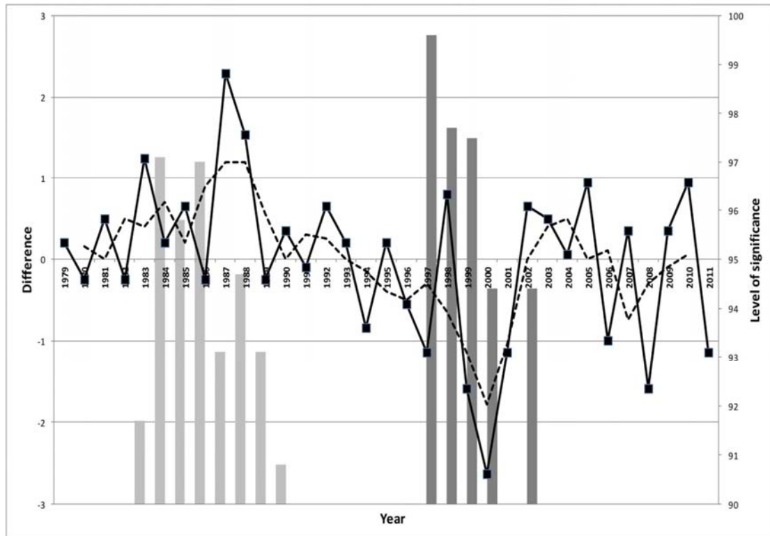
Fig. 7 Time series of normalized difference in zonal wind ( 40\text{-}15^{\circ}\text{S} minus 55\text{-}45^{\circ}\text{S} ) at 600 hPa (black solid line), 3-year moving average (broken line) and level of significance (secondary y-axis) exceeding 90% for moving 8-year above-average value (light grey bars) and 8-year below-average value (dark grey bars).
