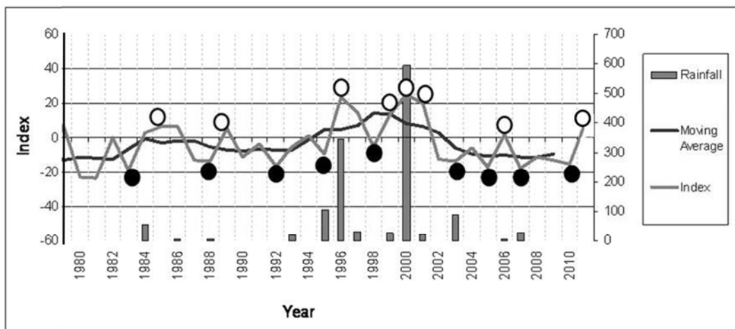
Fig. 4 Time series of the difference between the number of occurrences of Pattern B Positive and Pattern B Negative per JFM season (grey line, primary y-axis), 5-year moving average (black line) and annual rainfall (bars, secondary y-axis, units: mm) associated with tropical systems from the SWIO. El Niño and La Niña event years are indicated by solid and open circles, respectively.
