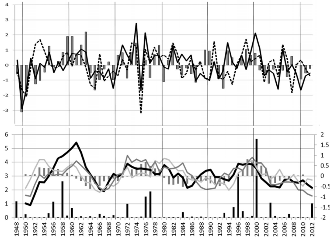
Fig. 12 Top: Detrended time series of the SAM (grey bars), normalized geopotential height anomaly (30-70°E, 45-25°S, solid line) and normalized zonal flow anomaly throughout 700 to 300 hPa (30-70°E: 45-15°S minus 55-45°S, broken line) for the 1948-2012 period. Bottom: 5-year filtered SAM (black line, secondary y-axis), normalized geopotential height anomaly at 250 hPa (dark grey line, secondary y-axis) and normalized zonal flow anomaly throughout 700 to 300 hPa (light grey line, secondary y-axis), 5-year filtered normalized total seasonal rainfall (grey bars, secondary y-axis) at all stations in the area of interest (Fig. 1) as well as average total rainfall per year contributed by tropical systems from the SWIO (black bars, primary y-axis, units: mm) over stations (dark circles in Fig. 1) in the Limpopo River Basin.
