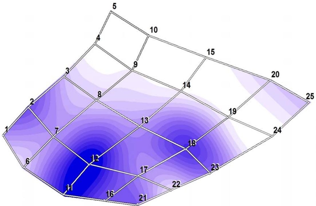
Fig. 2b As for Fig. 2a, but for 250 hPa.
