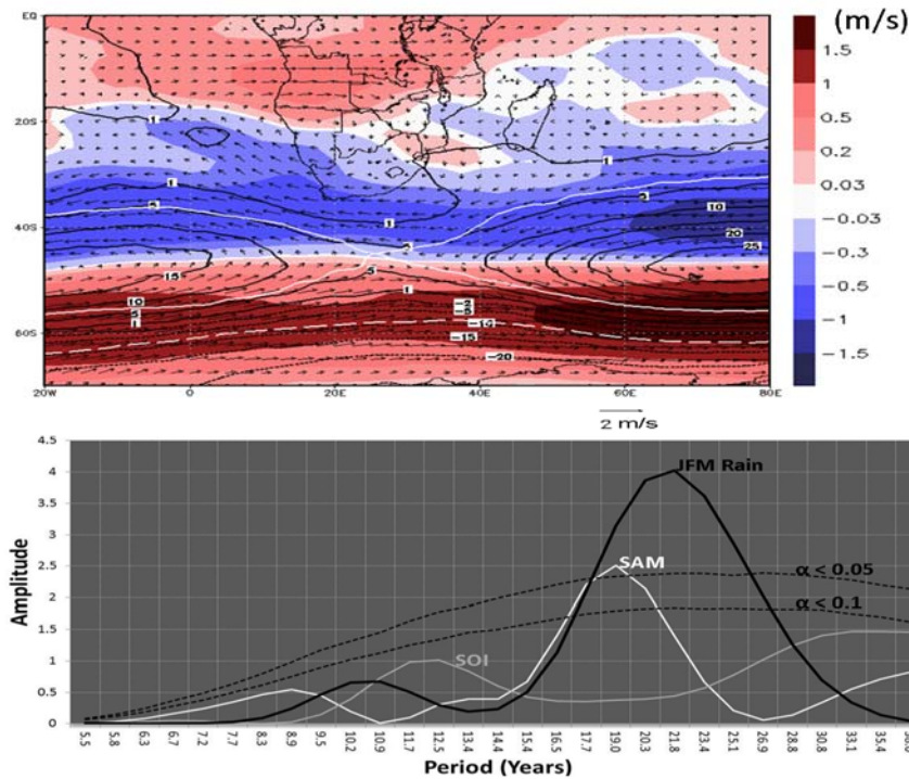
Fig. 13 The change (top) in JFM 250 hPa height (contours, units: m) and 500-700 hPa flow anomaly vectors (scale shown), with U-component shaded (red – positive, blue – negative, units: \text{ms}^{-1} ), per unit SAM increase. Areas where grid points indicate a local significant correlation with the SAM exceeding the 95% level of confidence is indicated by the white solid and broken lines for positive and negative correlations respectively. The period 1948-2011 is considered. The periodogram (bottom) is the result of a Fourier analysis over the same period based on the 5-year average of: the SAM (black line, primary axis), normalized SOI (grey line) and normalized rainfall (white line) at the stations in Fig. 1. Broken black lines are the 95% and 90% significance levels calculated for all three time series.
