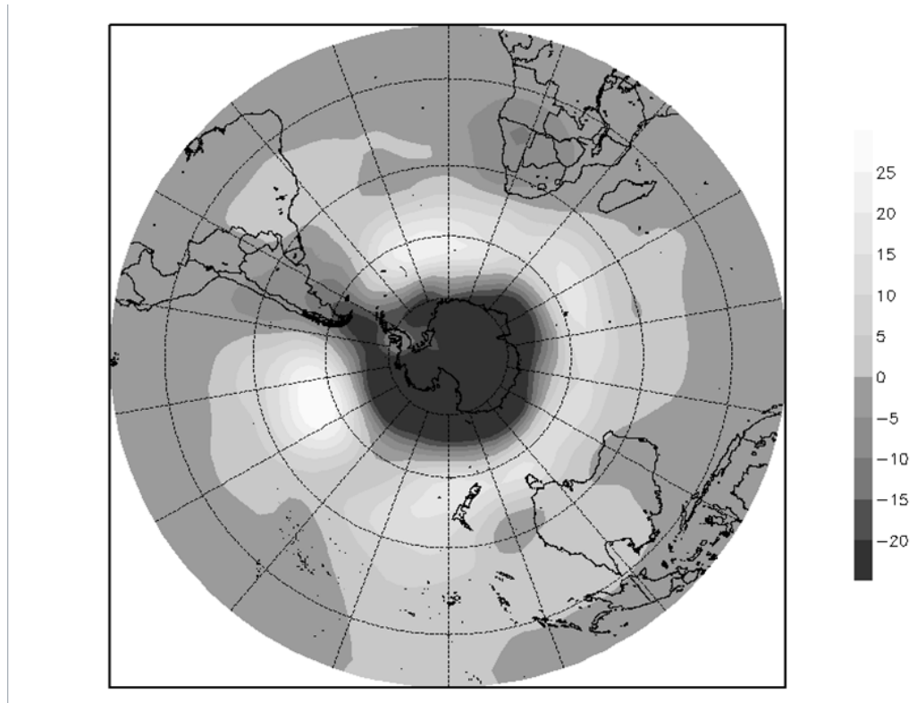
Fig. 11 Difference in 500 hPa geopotential heights (units: m) for 1995-2002 compared to the remaining years of the 1979-2011 period.
