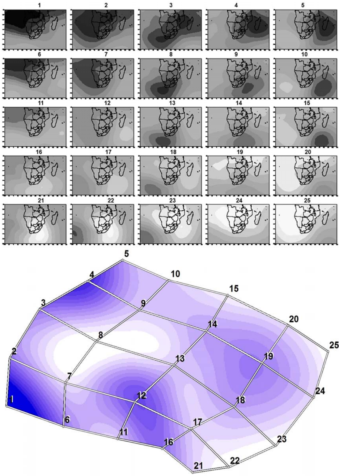
Fig. 2a SOM based on the standardized values with lighter (darker) shades showing positive (negative) deviations for the 850 hPa level (top), and Sammon map (bottom) showing the concentration of days associated with landfall and movement of tropical systems from the SWIO into the Limpopo River Basin for each SOM node. In the Sammon map, darker shades represent a higher concentration of days with landfall events. Numbers on the Sammon map correspond to the numbers of the nodes in the SOM. The 5 most favourable SOM nodes at this level are highlighted.
