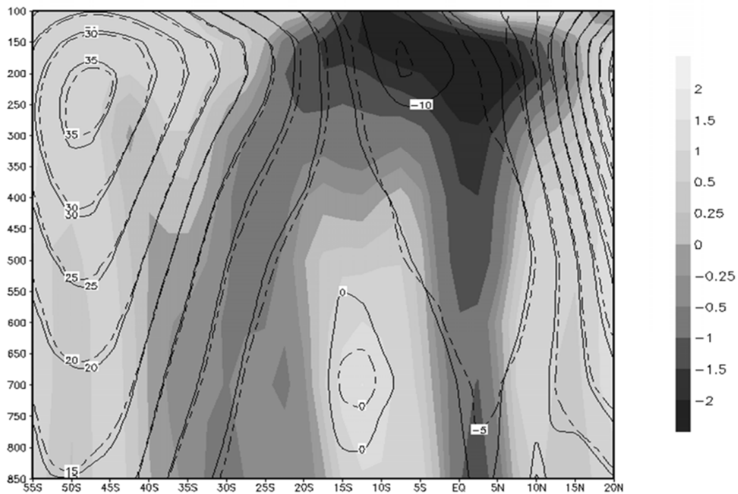
Fig. 6 Average zonal wind along 40°E during the 1995-2002 period (solid contours, units: \text{ms}^{-1} ), compared to the rest of the 1979-2011 period (dashed contours) and the difference (shaded).
