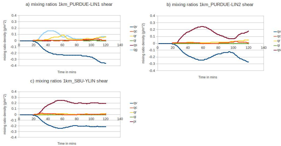
Figure 4.3.21: The change in mixing ratio with the a) PURDUE-LIN b) PURDUE-LIN with no graupel and c) SBU-YLIN microphysics scheme. A resolution of 1\text{ km} was used.
