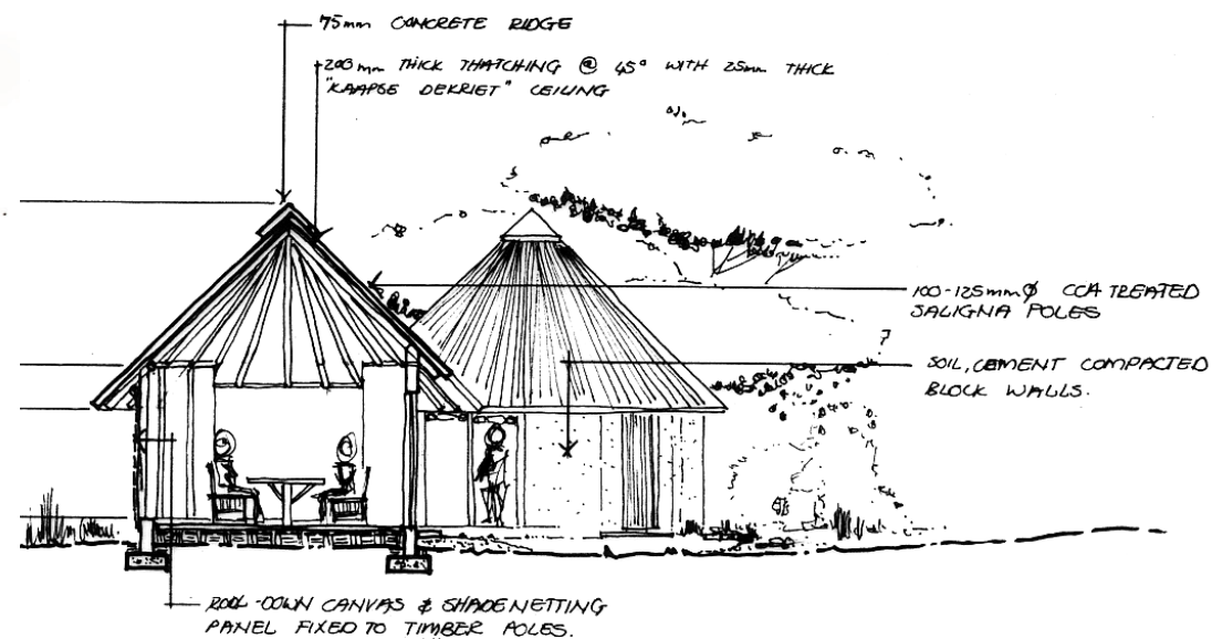
Fig. 8.12 Section through Break-away rooms
