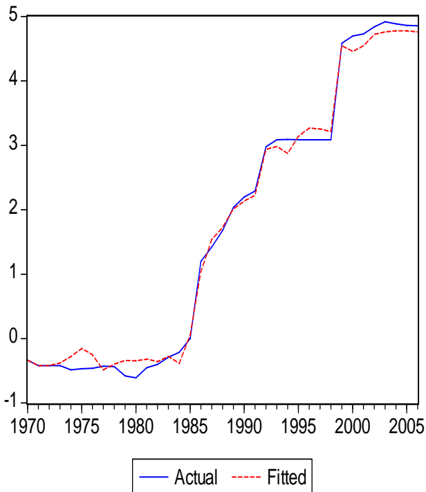
Figure 15: ln_exch
