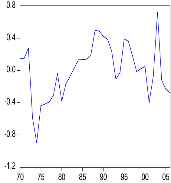
Figure 14: Residuals Infrastructure
