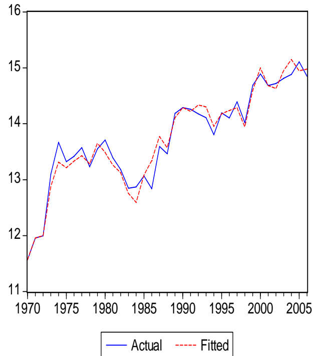
Figure 16: ln_rexp
