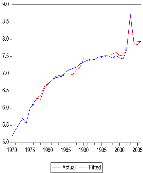
Figure 15: ln_exch
