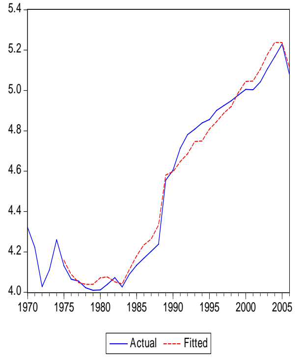
Figure 16: ln_rexp
