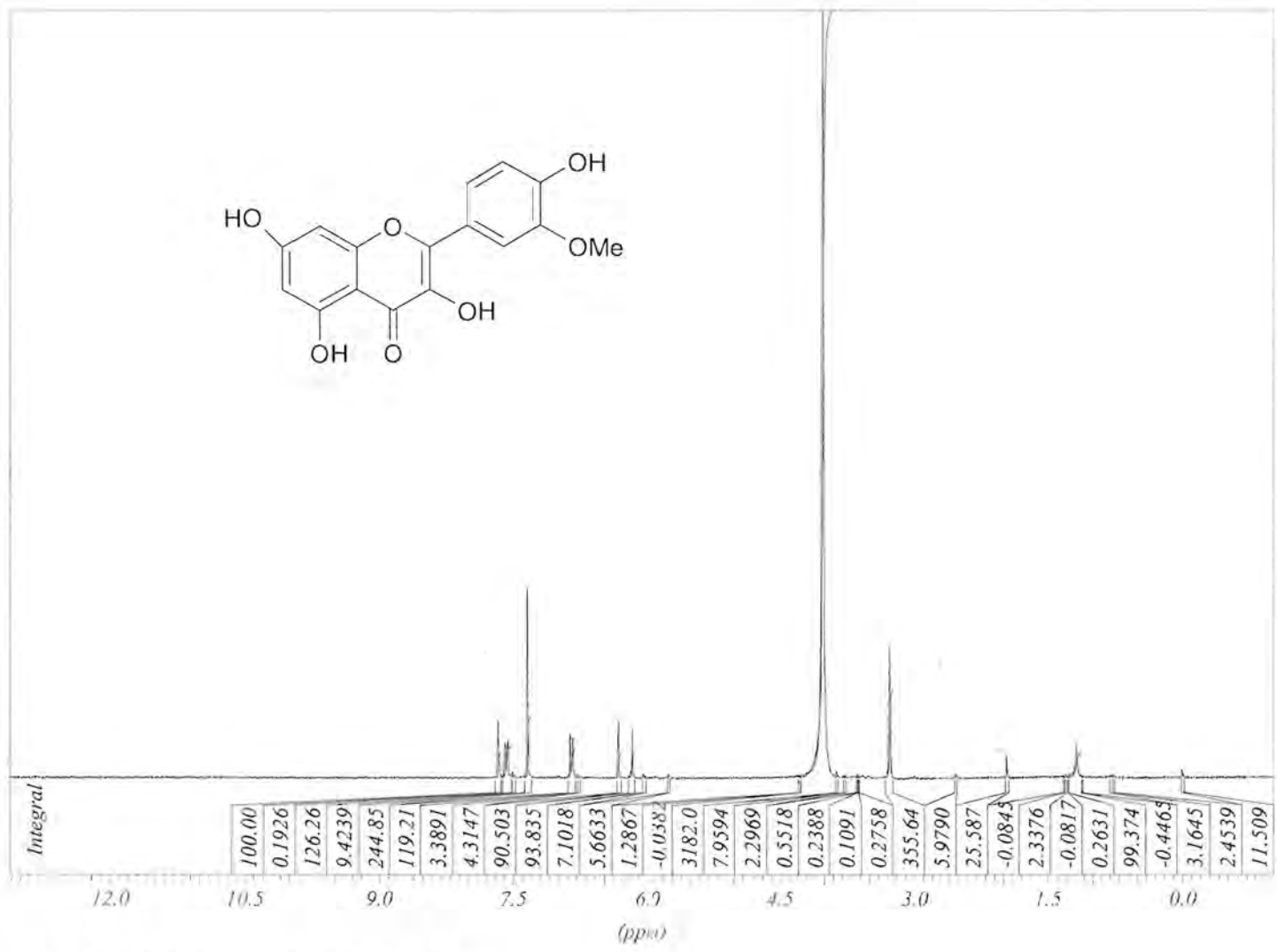
Figure 2.9: 1 H-NMR spectra of flavonoid 1.
