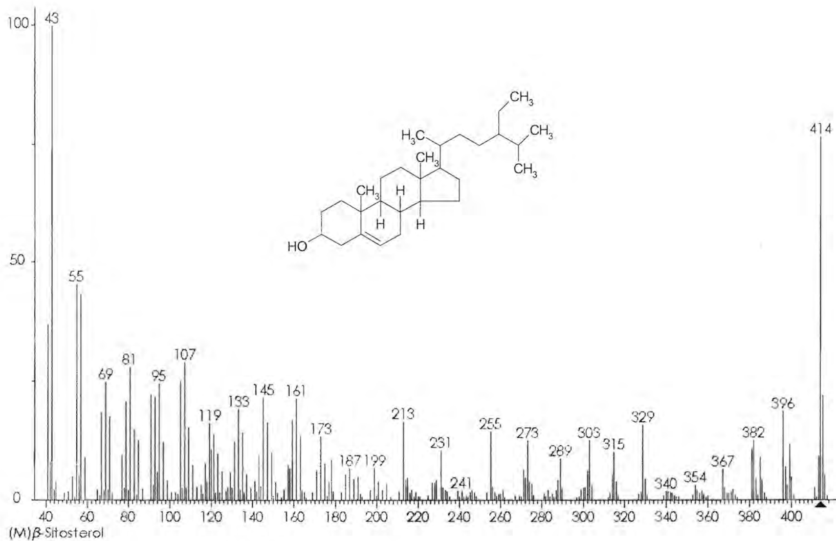
Figure 2.8: MS data of β-sitosterol from the MS-database.
