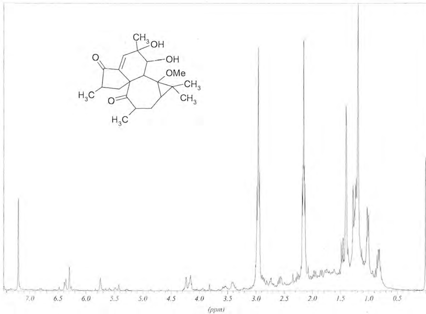
Figure 2.25: ^1\text{H-NMR} of diterpene 2.
