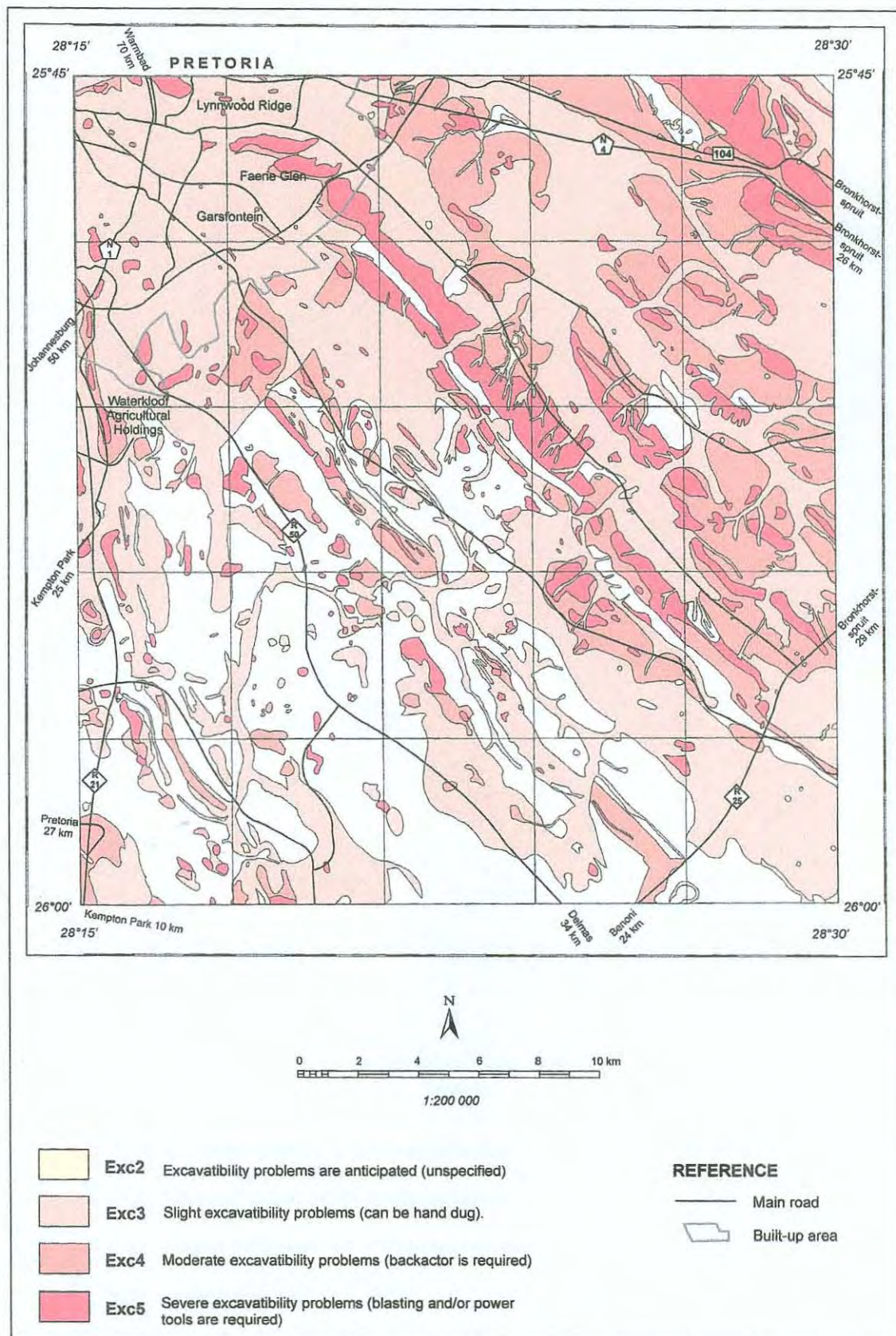
Figure 20: The excavability characteristics of the soil and the severity classes thereof in the Rietvleiam 2528 CD map sheet area
