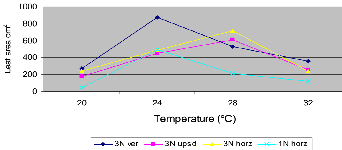
Figure 4.2 Interaction between temperature and orientation of cutting on leaf area per plant
