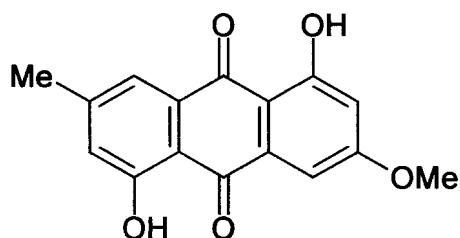
1,5-Dihydroxy-3-methoxy-7-methyl-anthraquinone
