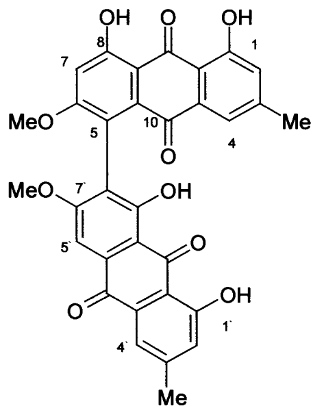
Floribundone
