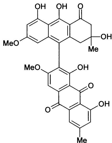
Anhydrophlegmic
