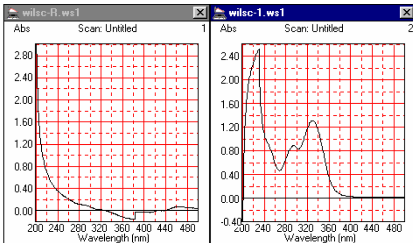
Figure B8: Absorption spectrum of SC1 in NaOAc + H 3 BO 3
