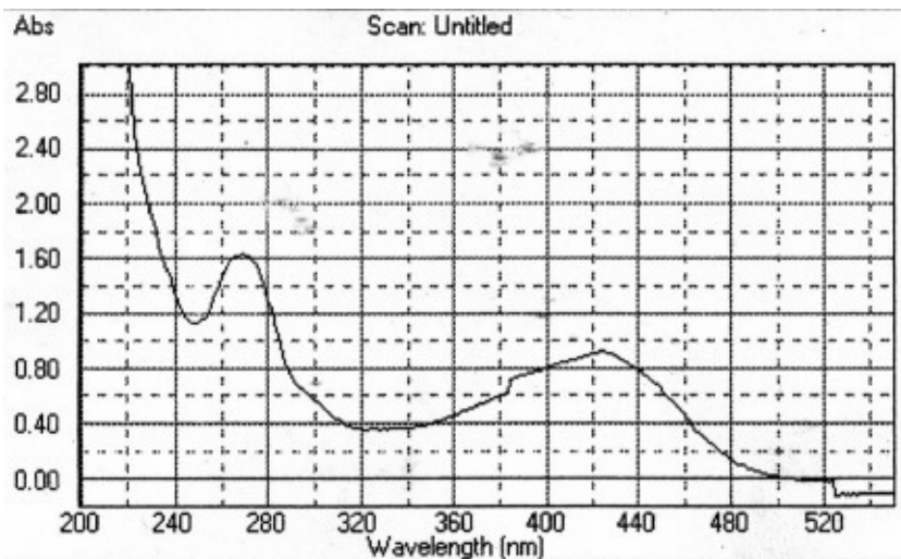
Figure A3: Absorption spectrum of PC1 in methanol and \text{AlCl}_3
