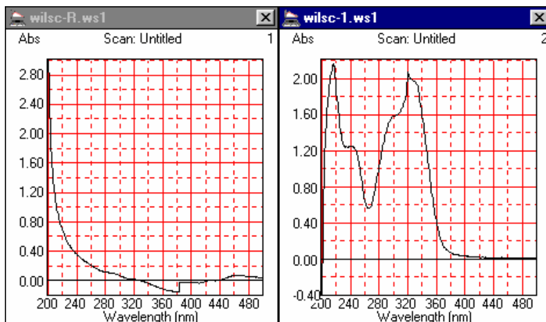
Figure B10: Absorption spectrum of SC2 in MeOH
