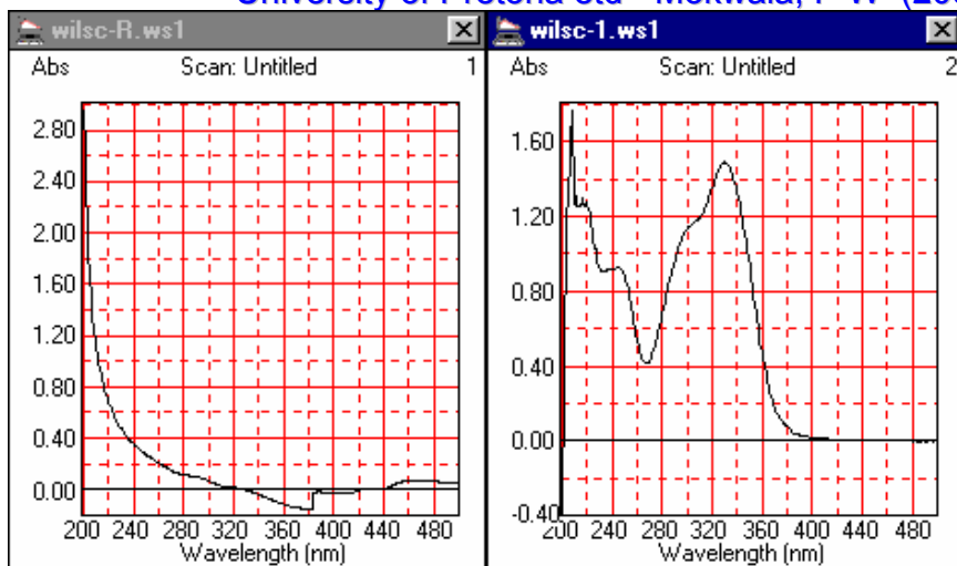
Figure B5: Absorption spectrum of SC1 in AICI + HCl
