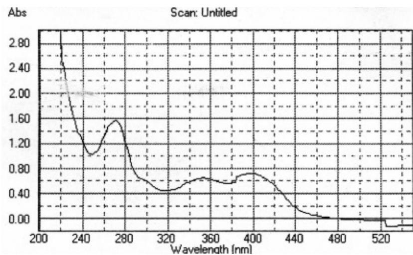
Figure A4: Absorption spectrum of PC1 in methanol \text{AlCl}_3 and HCl
