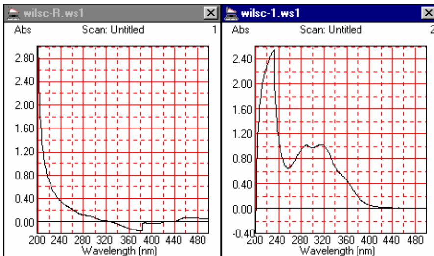
Figure B6: Absorption spectrum of SC1 in MeOH + NaOAc
