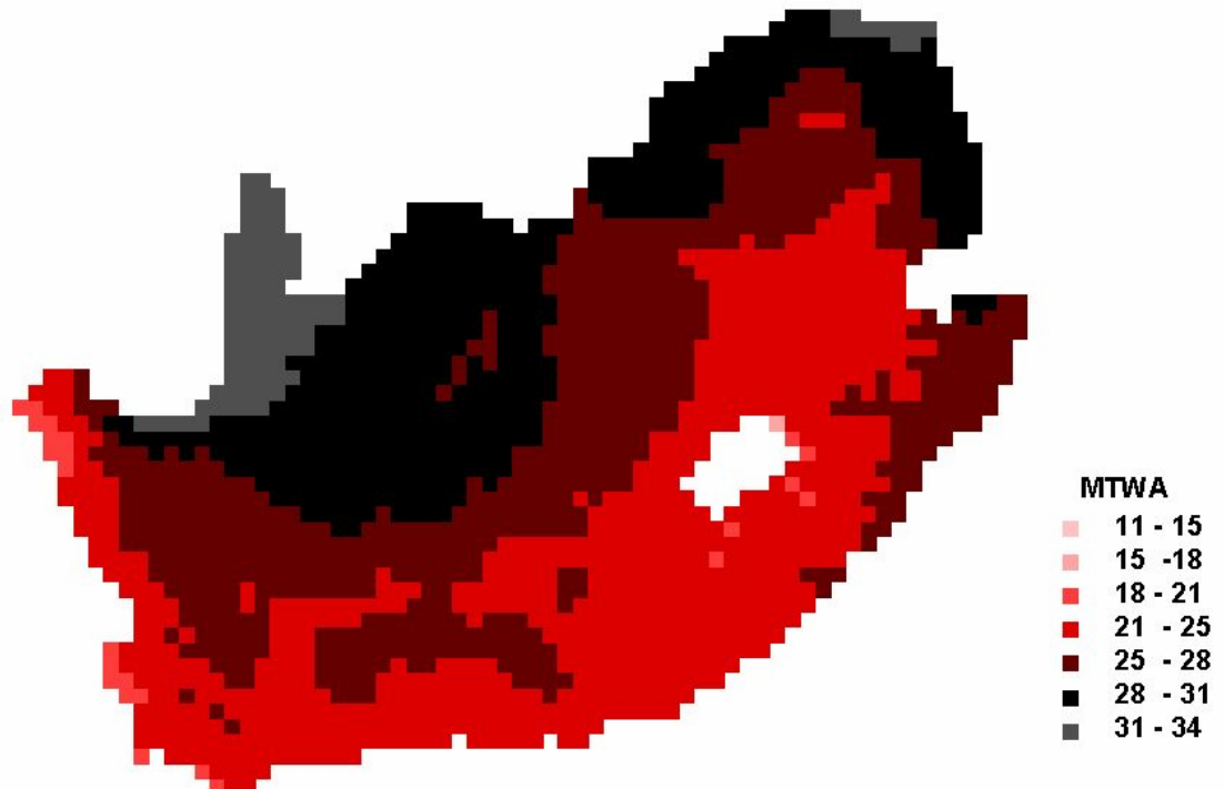
Figure B.11 — Mean temperature of the warmest month values ( ^{\circ}\text{C} ) values calculated for the SCT data using the future climate represented by the HadCM3 B2 scenario.
