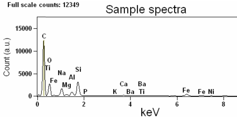
Figure 2-37: Example of an EDS spectrum
