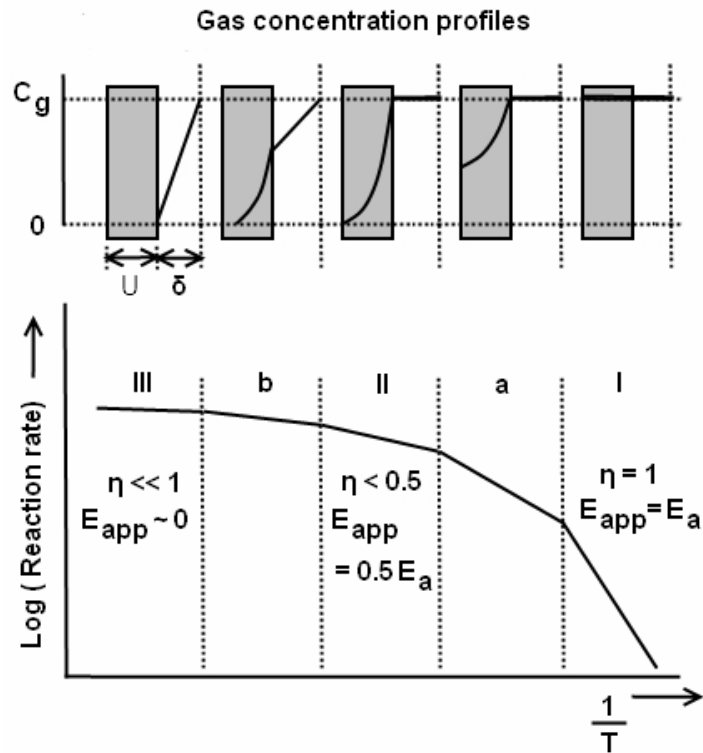
Figure 2-49: Gas-carbon reaction zones
