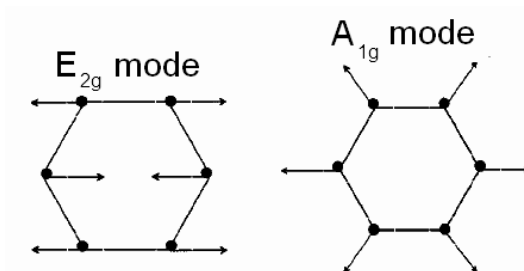
Figure 2-35: Raman active modes for graphite
