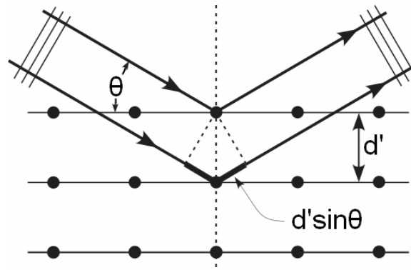
Figure 2-31: Electromagnetic beam incident on a crystal lattice
