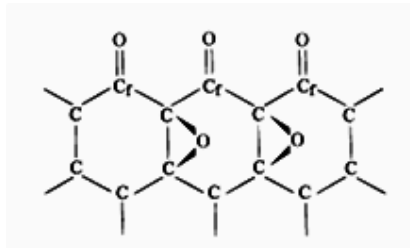
Figure 2-54: Off-plane oxygen surface complex
