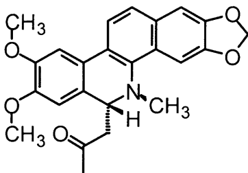
8-acetyldihydroneurine
